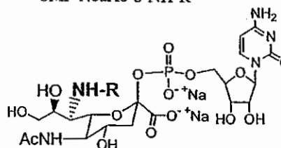
CMP-NeuAc-8-NH-R
