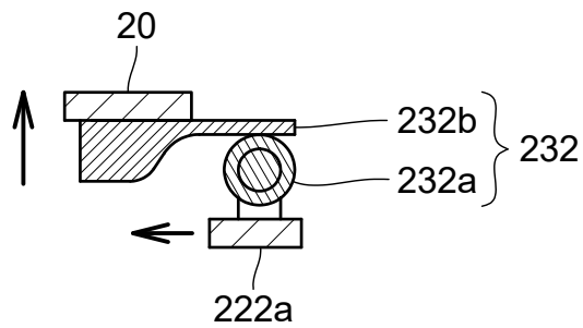
CROSS-SECTIONAL VIEW ACROSS A LINE A-A (VERTICAL CAM MECHANISM)
