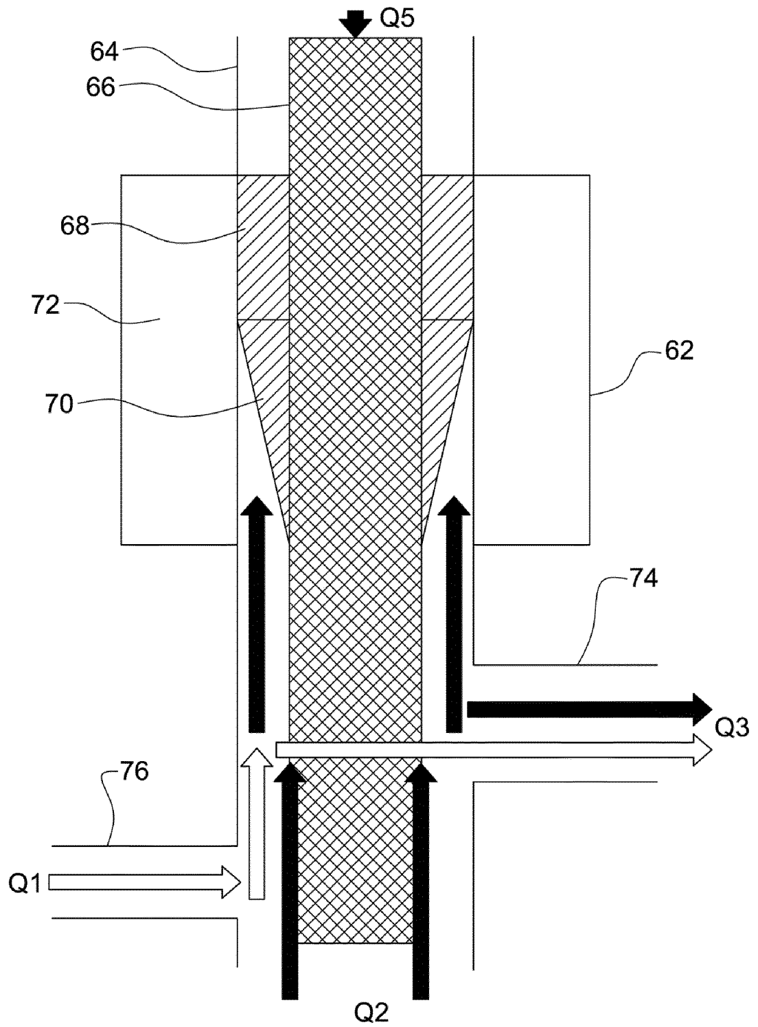
FIG 6 (PRIOR ART)
