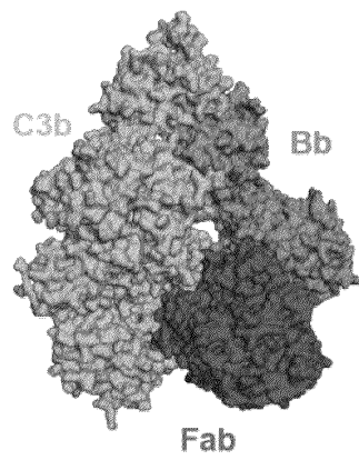
Trimeric complex: C3bBb + Fab
