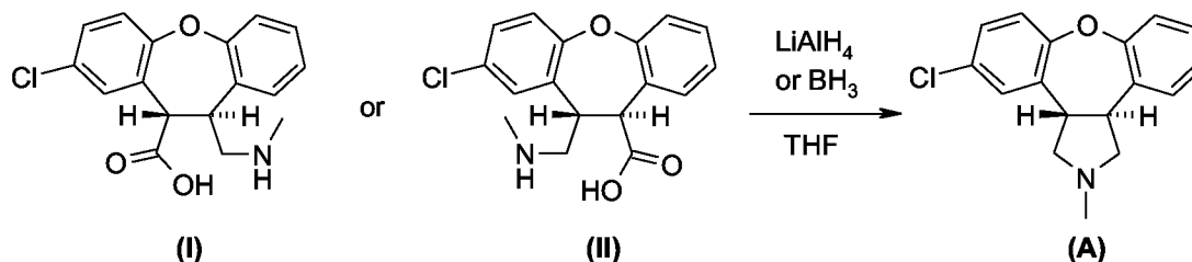
Scheme V
