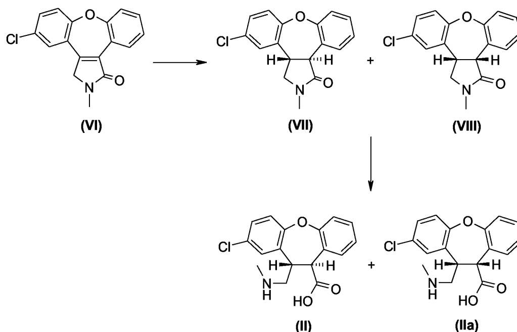
Scheme IV
