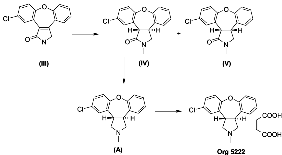
Scheme I
