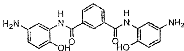
Hydroxyl group-containing diamine (c)
