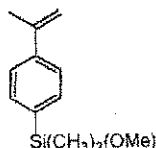
\alpha -methylstyryl dimethylmethoxysilane
