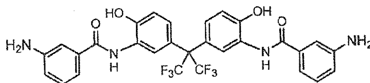
Hydroxyl group-containing diamine (b)
