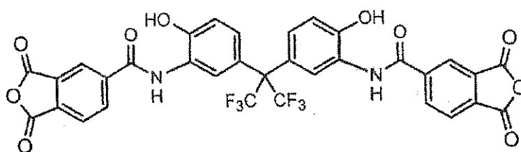
Hydroxyl group-containing acid anhydride (a)
