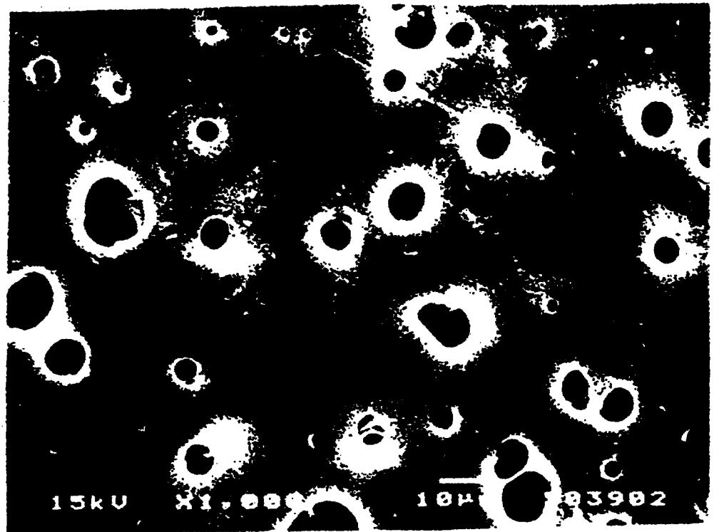
SEM Photo 5 of Polysulfone Membrane Surface(Tight side) @ Magnification = 1,000 X
