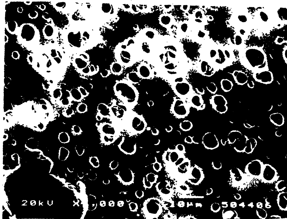
SEM Photo 6 of Polysulfone Membrane Surface(Tight side) @ Magnification = 1,000 X
