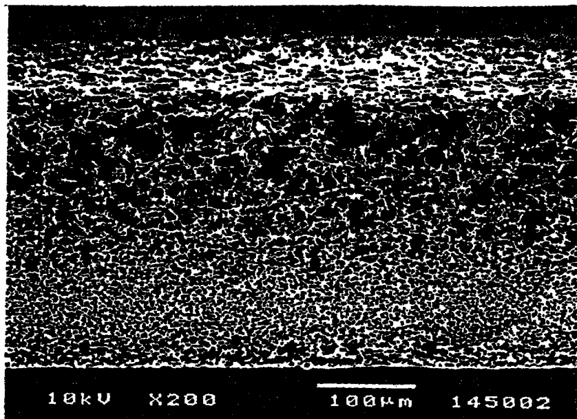
Cross-section @ Magnification = 200 X
