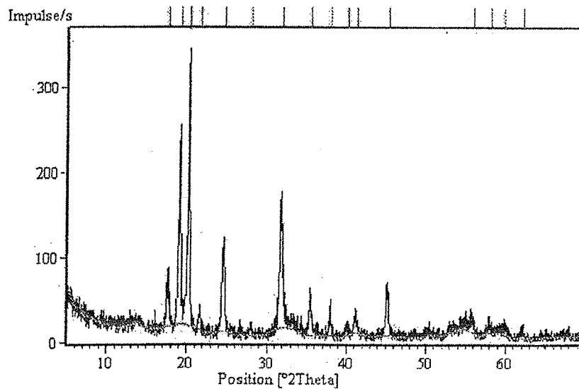
Figure 1b: an XRD spectrum of the iron (III) orthophosphate of Figure 1a.
