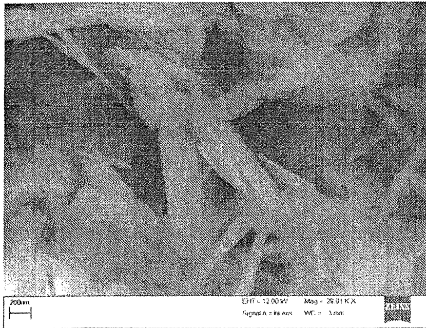
Figure 2a: a scanning electron microscope image of iron (III) orthophosphate according to the invention produced from \text{Fe}_3\text{O}_4 in accordance with Example 1 which is present predominantly in the metastrengite II crystal structure.
