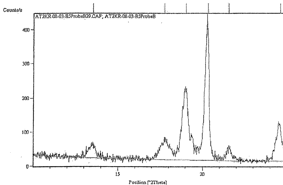
Figure 2b: an XRD spectrum of the iron (III) orthophosphate of Figure 2a.
