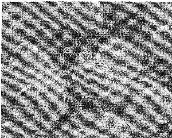
Figure 1a: a scanning electron microscope image of an iron (III) orthophosphate with a metastrengite I crystal structure produced in accordance with a known process in accordance with the state of the art from \text{Fe(II)SO}_4 .
