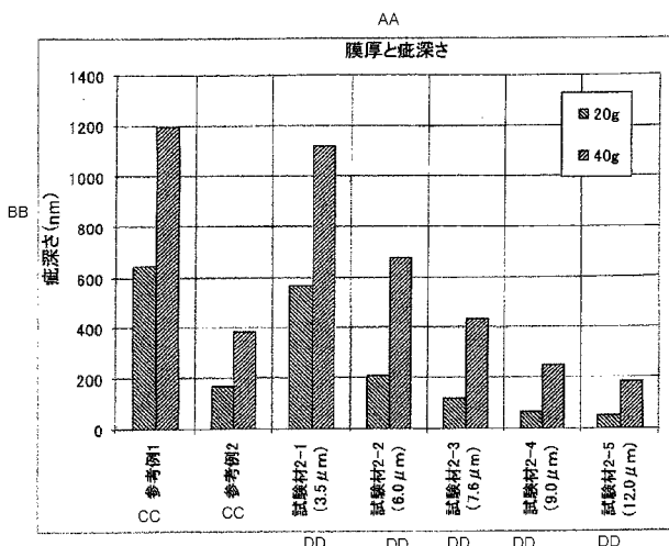
FIG. 3: AA Film thickness and depth of scratch BB Depth of scratch (nm) CC Reference example DD Test material
