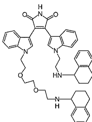
Compound 29a
