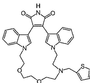
Compound 23a
