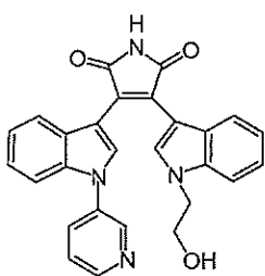
Compound 1a
