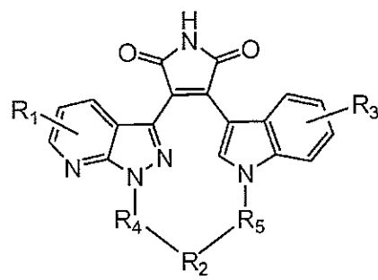
Formula (IIIl)
