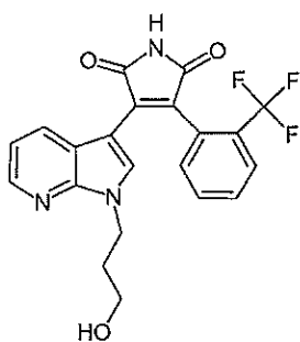
Compound 11
