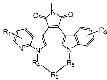
Formula (IIIj)
