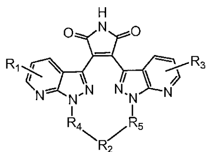
Formula (IIId)
