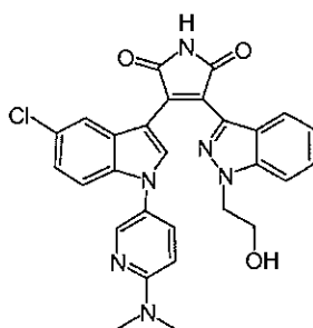
Compound 31a
