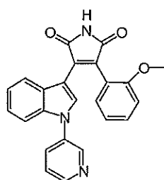
Compound 2a
