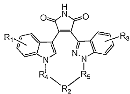
Formula (IIIf)
