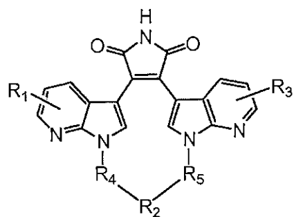
Formula (IIIb)
