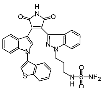
Compound 10a
