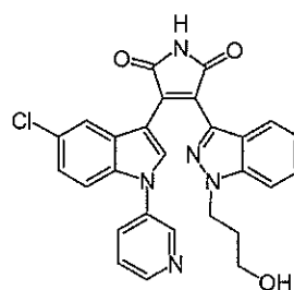
Compound 12a
