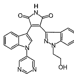
Compound 12a
