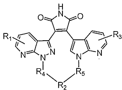
Formula (IIIh)
