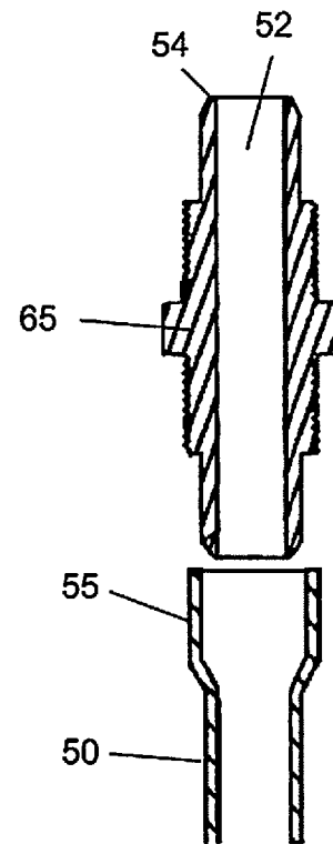
FIG. 1C (PRIOR ART)
