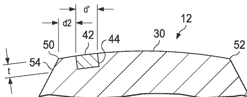
FIG. 4 (PRIOR ART)
