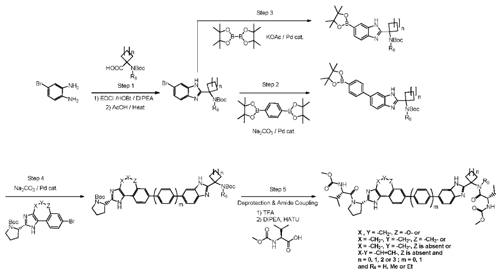
Scheme I
