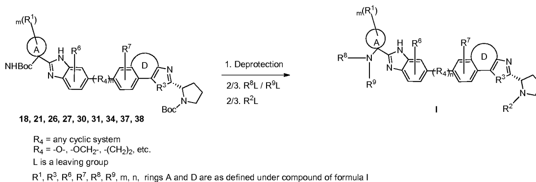
Scheme 11:
