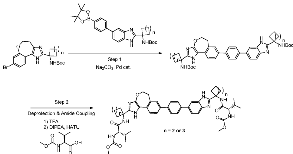
Scheme II
