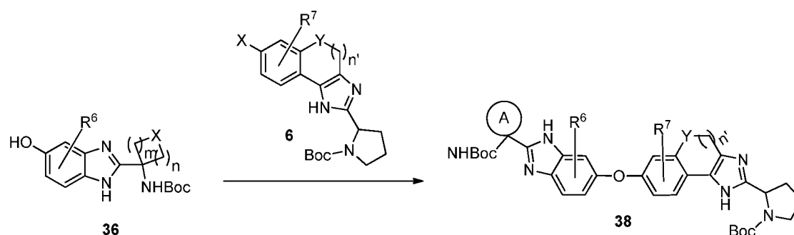
Scheme 10:
