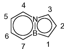
3a,7a-azaborindenyl
