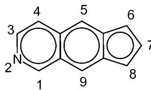
cyclopenta[g]isoquinolyl
