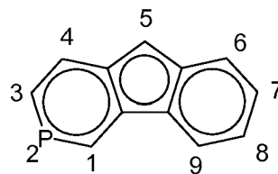
indeno[1,2-c]phosphinyl
