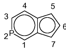
cyclopenta[c]phosphinyl
