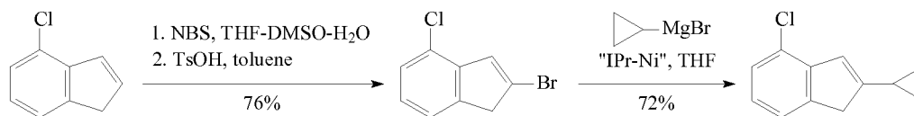
Scheme B:
