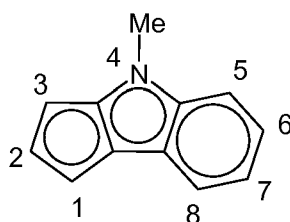
4-methylcyclopenta[ b ]indolyl
