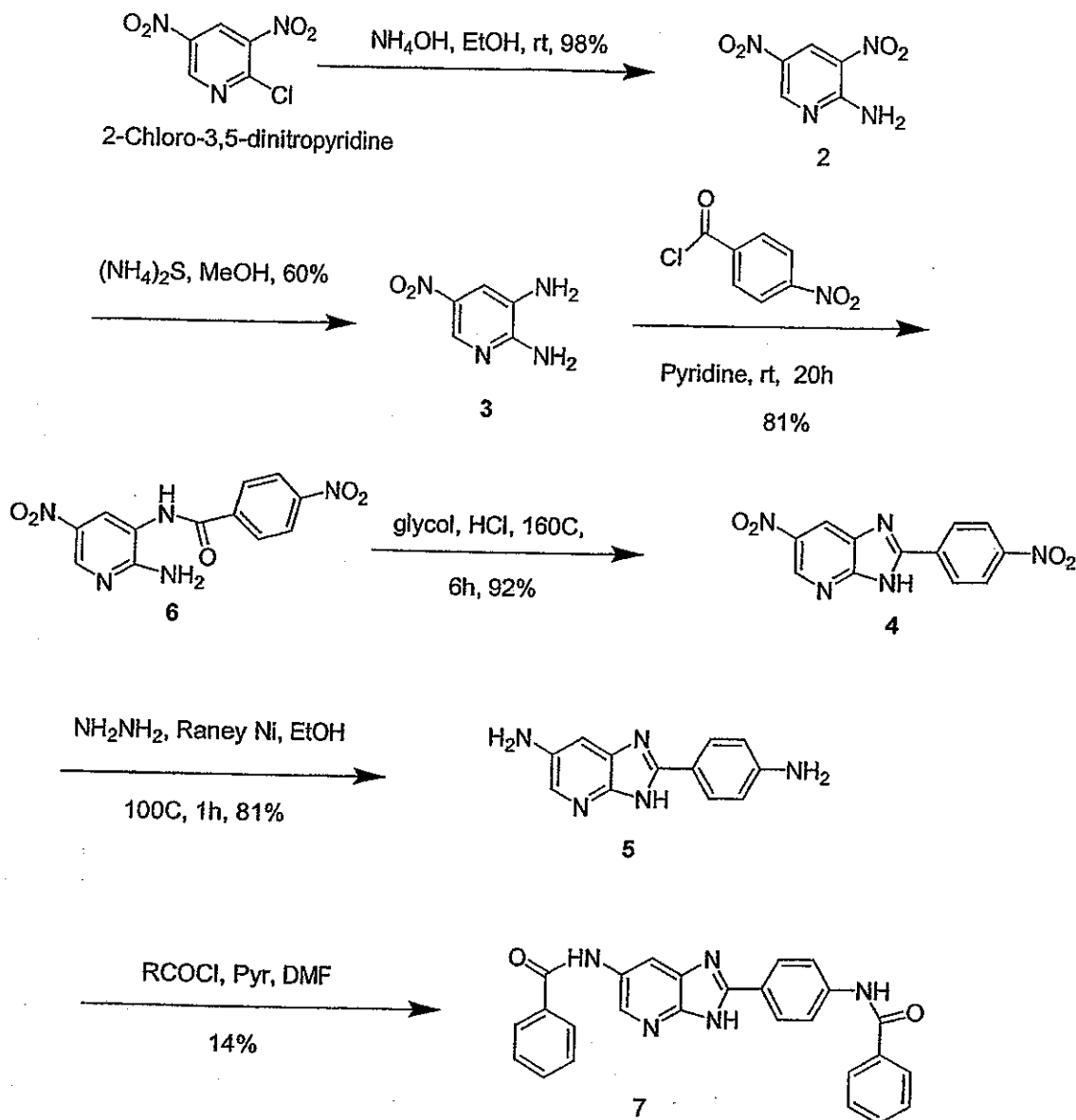
Scheme 36
