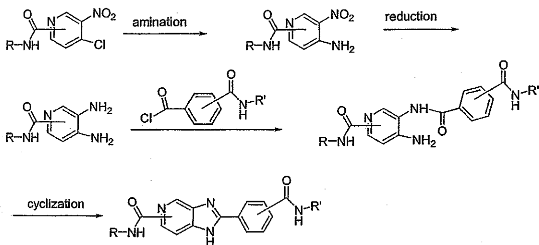
Synthetic Scheme 15
