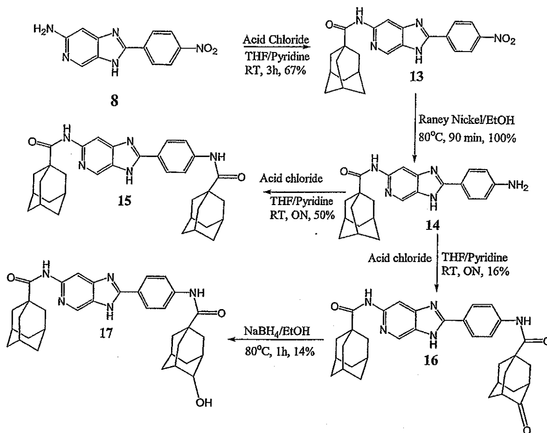
Scheme 39
