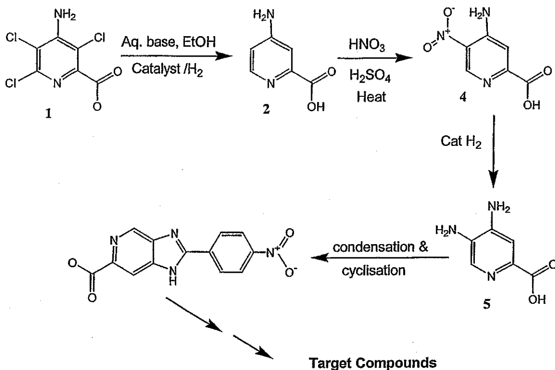
Scheme 44
