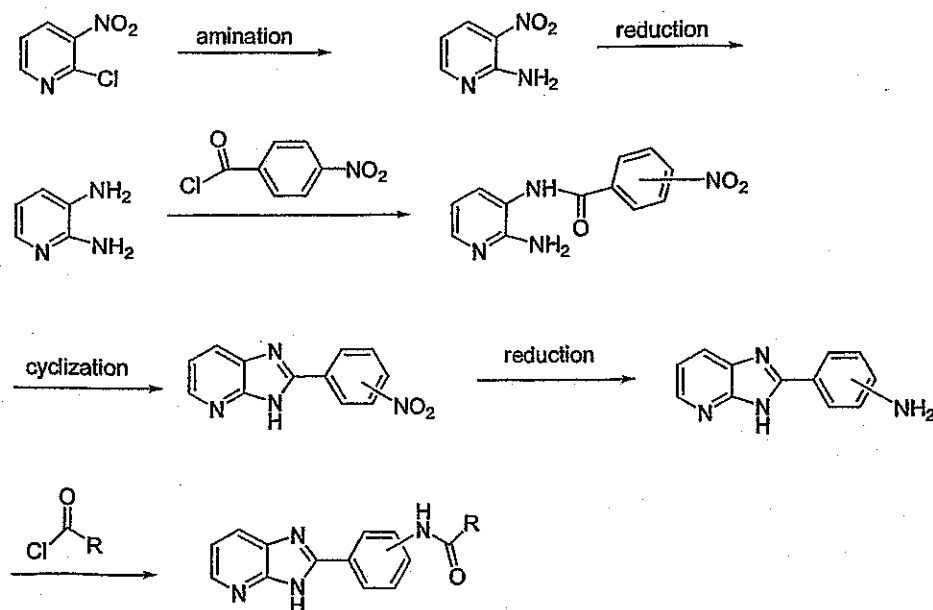
Synthetic Scheme 9
