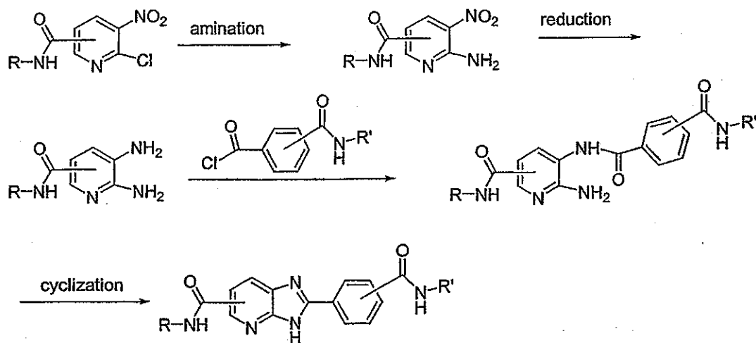
Synthetic Scheme 11
