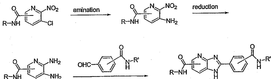
Synthetic Scheme 18
