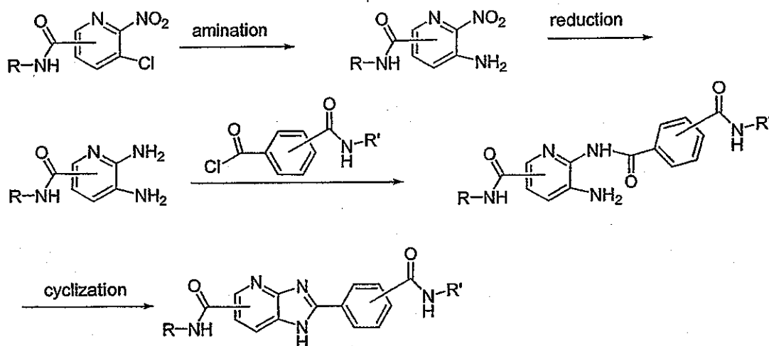
Synthetic Scheme 17
