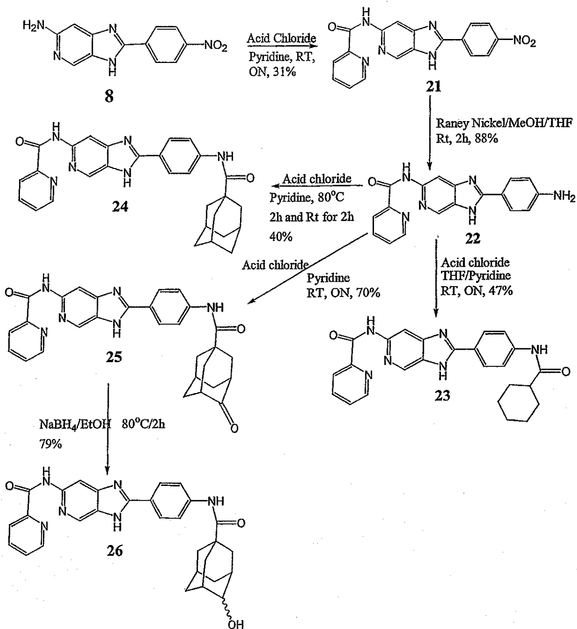
Scheme 41
