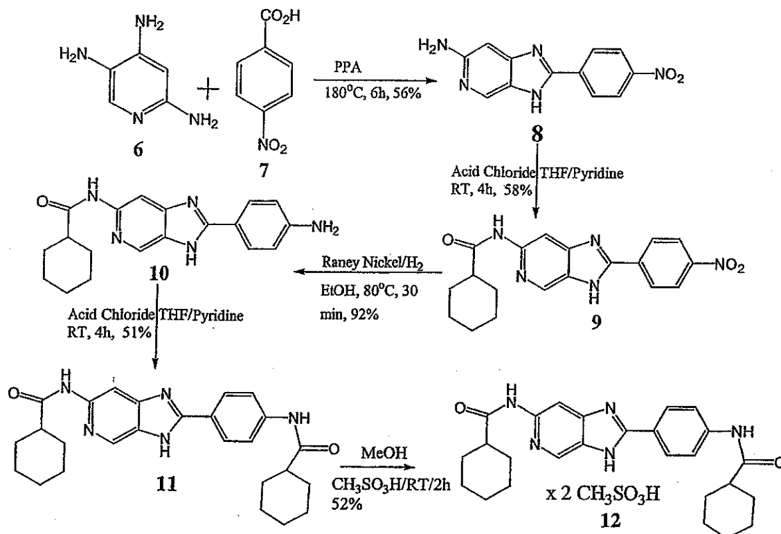
Scheme 38
