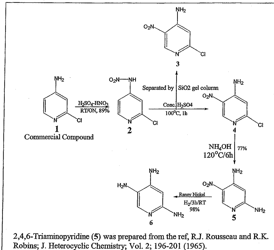
Scheme 37
