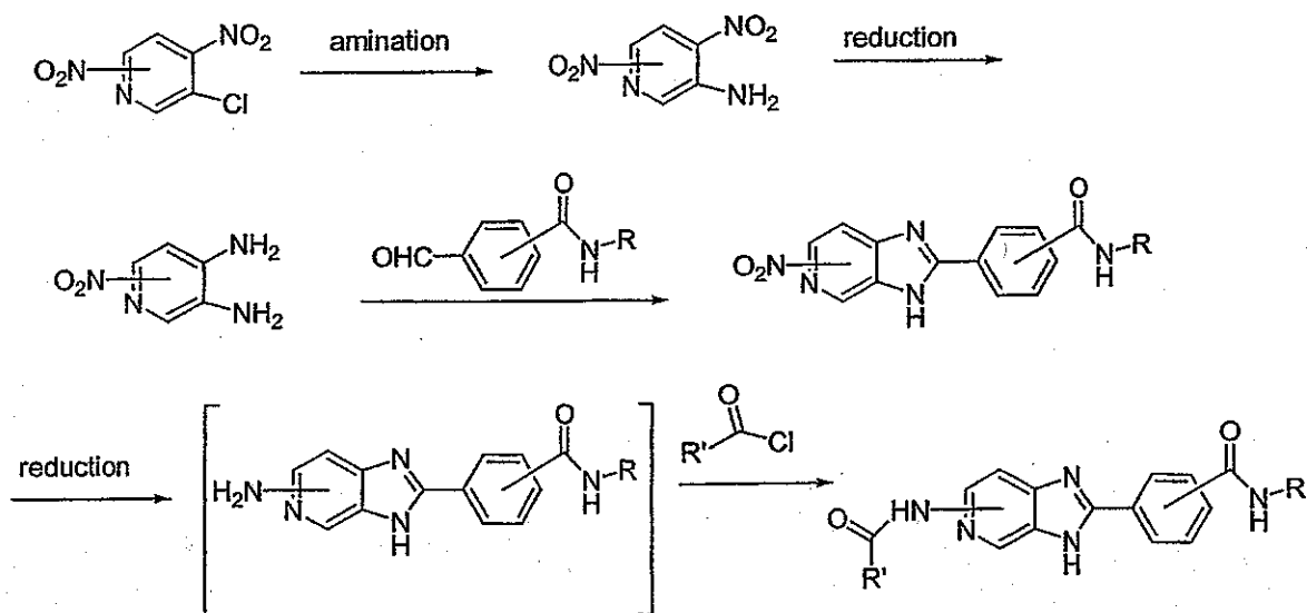
Synthetic Scheme 22
