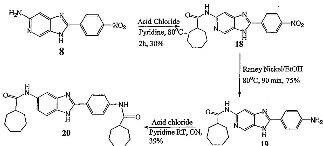
Scheme 40
