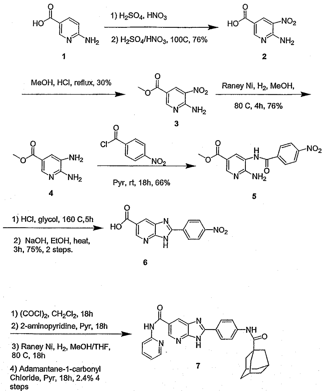
Scheme 42
