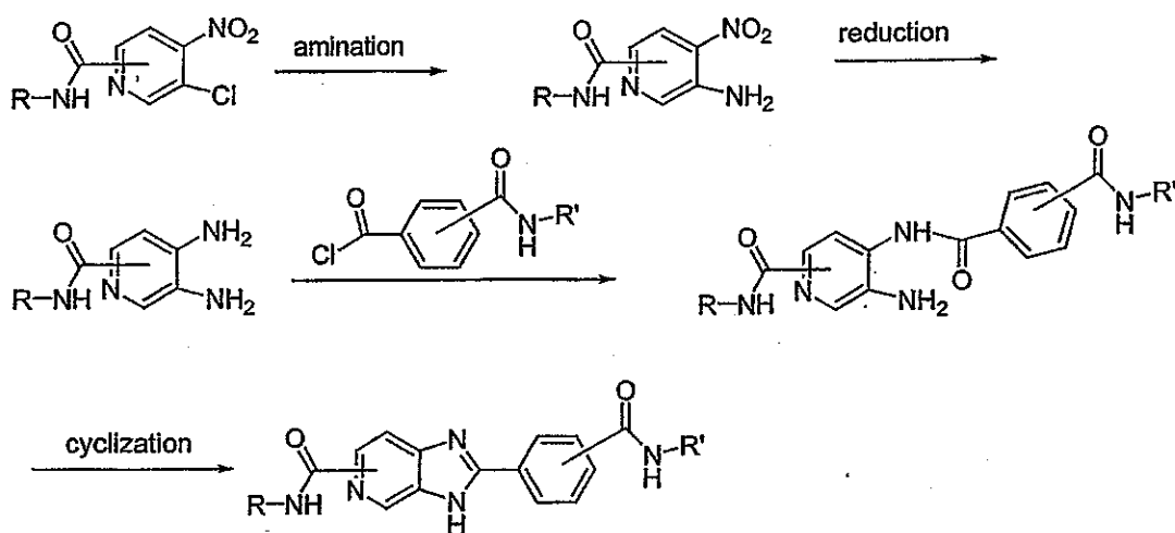
Synthetic Scheme 13
