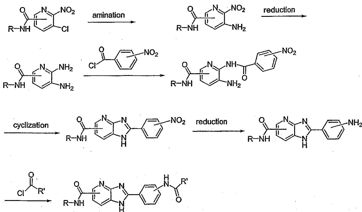
Synthetic Scheme 7
