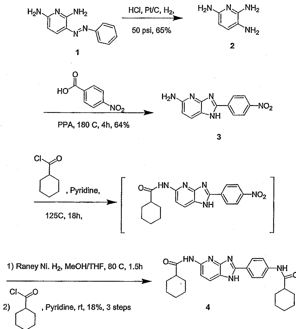
Scheme 43
