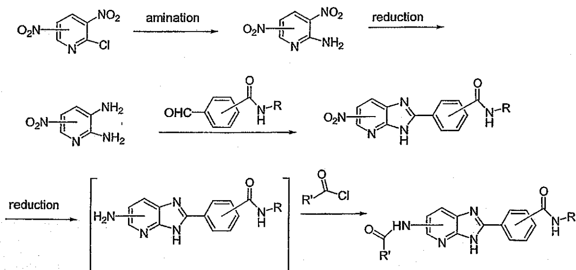
Synthetic Scheme 20
