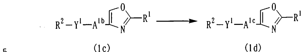
Reaction Scheme 4
