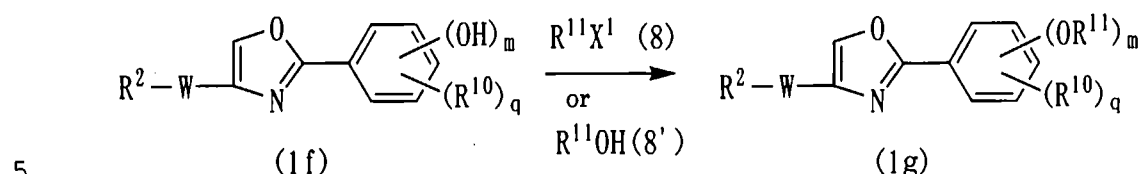
Reaction Scheme 6
