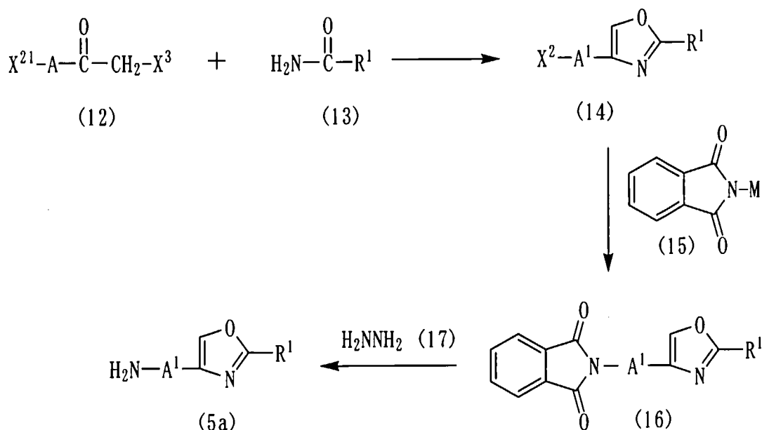
Reaction Scheme 10
