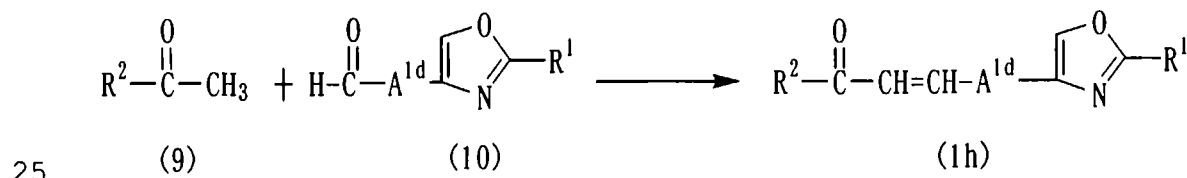
Reaction Scheme 7
