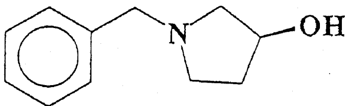
(S)-N-Benzyl-3-pyrrolidinol
