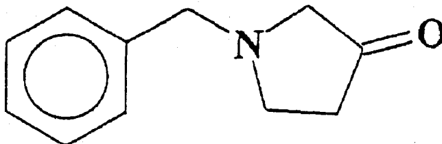
N-Benzyl-3-pyrrolidinone
