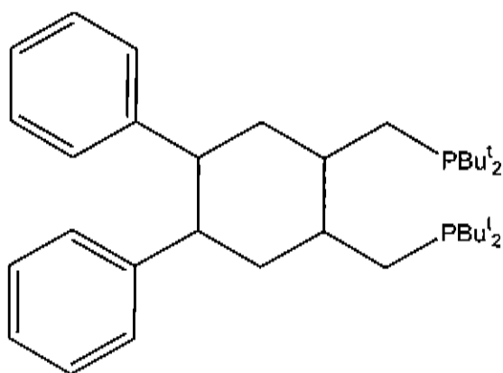
10 cis-1,2 bis(di- tert -butyl(phosphinomethyl))-4,5 diphenyl cyclohexane
