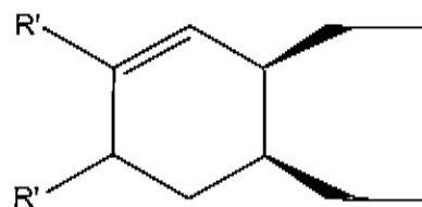
1 and/or 6 - substituted cyclohexenyl
