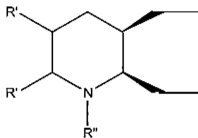
5 and/or 6 substituted piperidines
