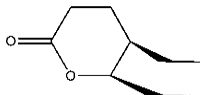
delta-valero lactone 4,5-diyl
