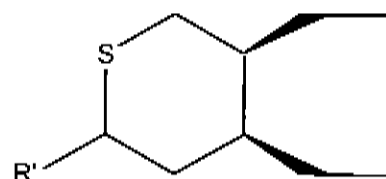
substituted pentamethylene sulphide (substituted tetrahydro-thiopyran)
