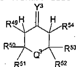
(IIIc)
