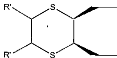
2 and/or 3 substituted 1,4 dithiane
