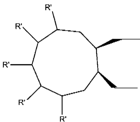
4,5,6,7 and/or 8 substituted cyclononyl
