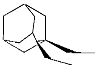
Adamantyl -1,2-diyl
