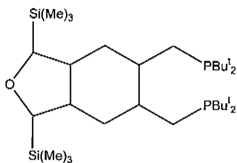
20 cis-5,6-bis(di- tert -butylphosphinomethyl)-1,3-bis(trimethylsilyl)-3a,4,5,6,7,7a-hexahydro-1,3H-isobenzofuran.
