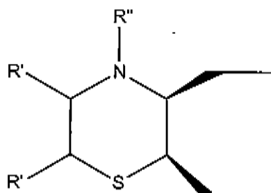
10 1, 2, 3, 4 substituted piperazine
