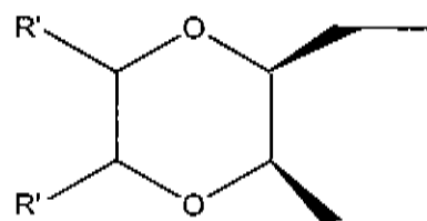
5 and/or 6 substituted 1,4 dioxane
