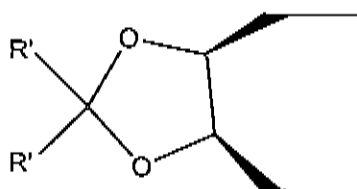
5 substituted DIOP
