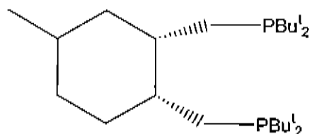
cis- 1, 2-bis (di- tert -butylphosphinomethyl) 5-methylcyclohexane
