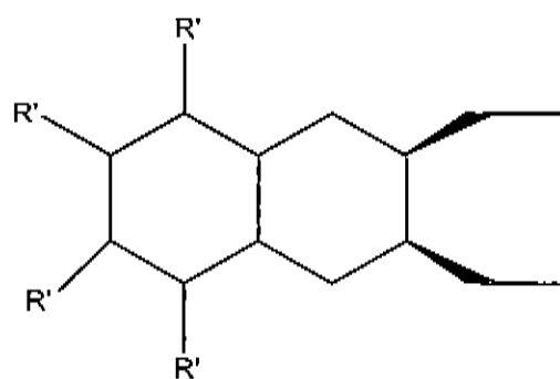
2,3,4 and/or 5 substituted decahydronaphthalene
