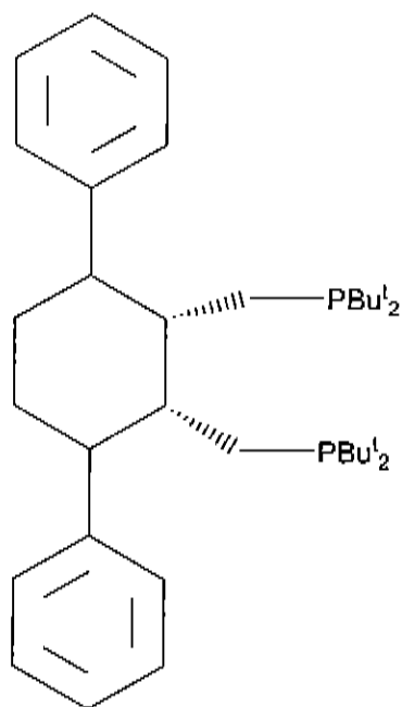
5 cis-1, 2-bis (di-tert-butylphosphinomethyl), 3, 6, diphenylcyclohexane
