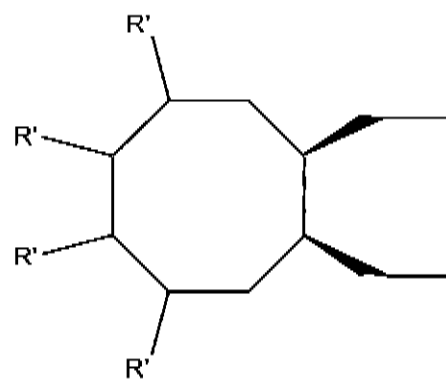
4, 5, 6 and/or 7 substituted cyclooctyl
