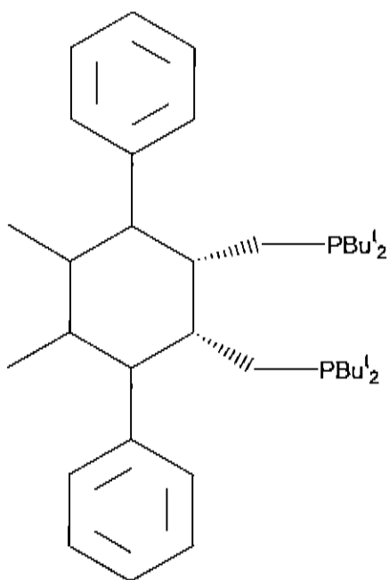
cis-1, 2-bis (di-tert-butylphosphinomethyl), 3, 6, diphenyl-4,5 dimethyl-cyclohexane
