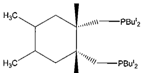
cis-1, 2-bis (di-tert-butylphosphinomethyl), 1, 2, 4, 5 tetramethylcyclohexane
