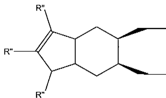
substituted 3a, 4,5,6,7,7a
