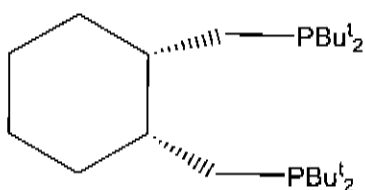
cis- 1, 2-bis (di-tert-butylphosphinomethyl) cyclohexane
