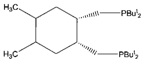
cis-1, 2-bis (di-tert-butylphosphinomethyl), 4, 5 dimethylcyclohexane
