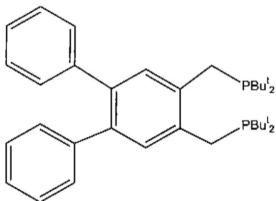
10 1,2bis(di-tert-butyl(phosphinomethyl)-4,5-diphenyl benzene
