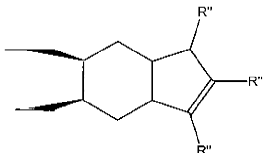
Substituted 3a, 4,5,6,7,7a-hexahydro-1H-indene
