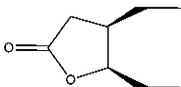
gamma-butyrolactone
