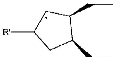
4 substituted cyclopentyl
