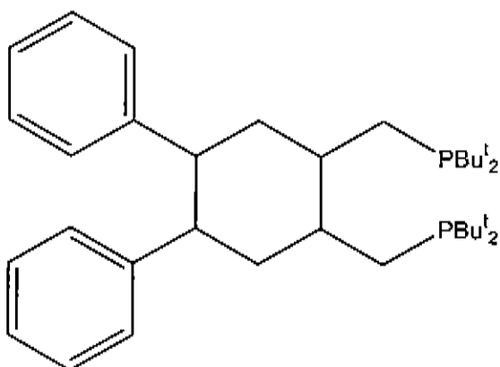
cis-1,2 bis(di-tert-butyl(phosphinomethyl)-4,5 diphenyl cyclohexane
