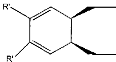
2 and/or 3 substituted cyclohexadienyl
