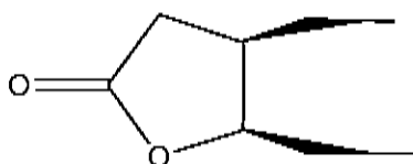
15 tetrahydro-furan-2-one
