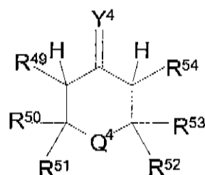
(IIIId)
