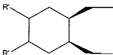
40 4 and/or 5 substituted cyclohexyl
