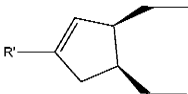
15 1 - substituted cyclopentenyl
