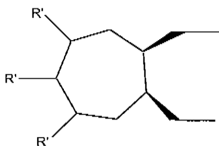
4, 5 and/or 6 substituted cycloheptyl
