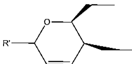
10 Substituted dihydropyran
