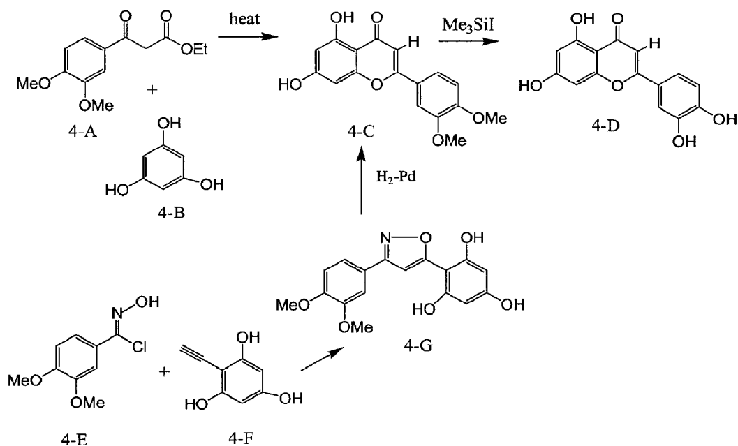
Scheme 4. Alternative Routes to Flavone analogs.
