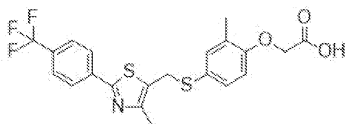
GW501516
