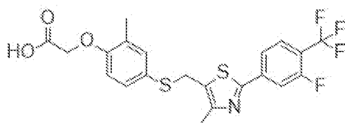
GW0742
