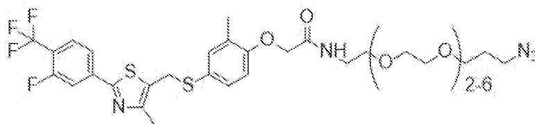
GW0742-Amide derivative
