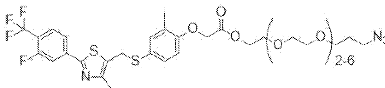
GW0742-Ester-derivative
