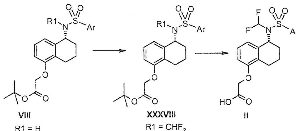
Scheme 8
