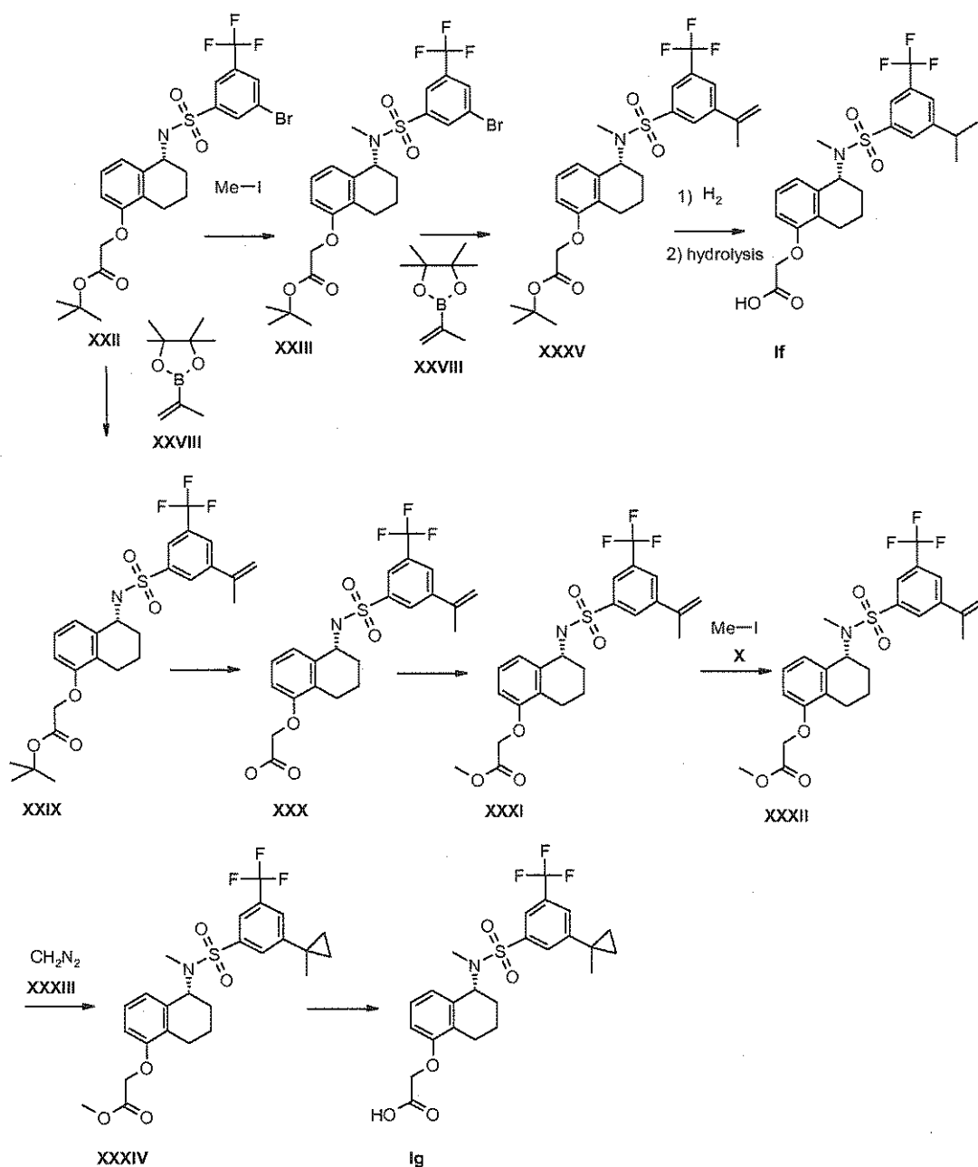
Scheme 6
