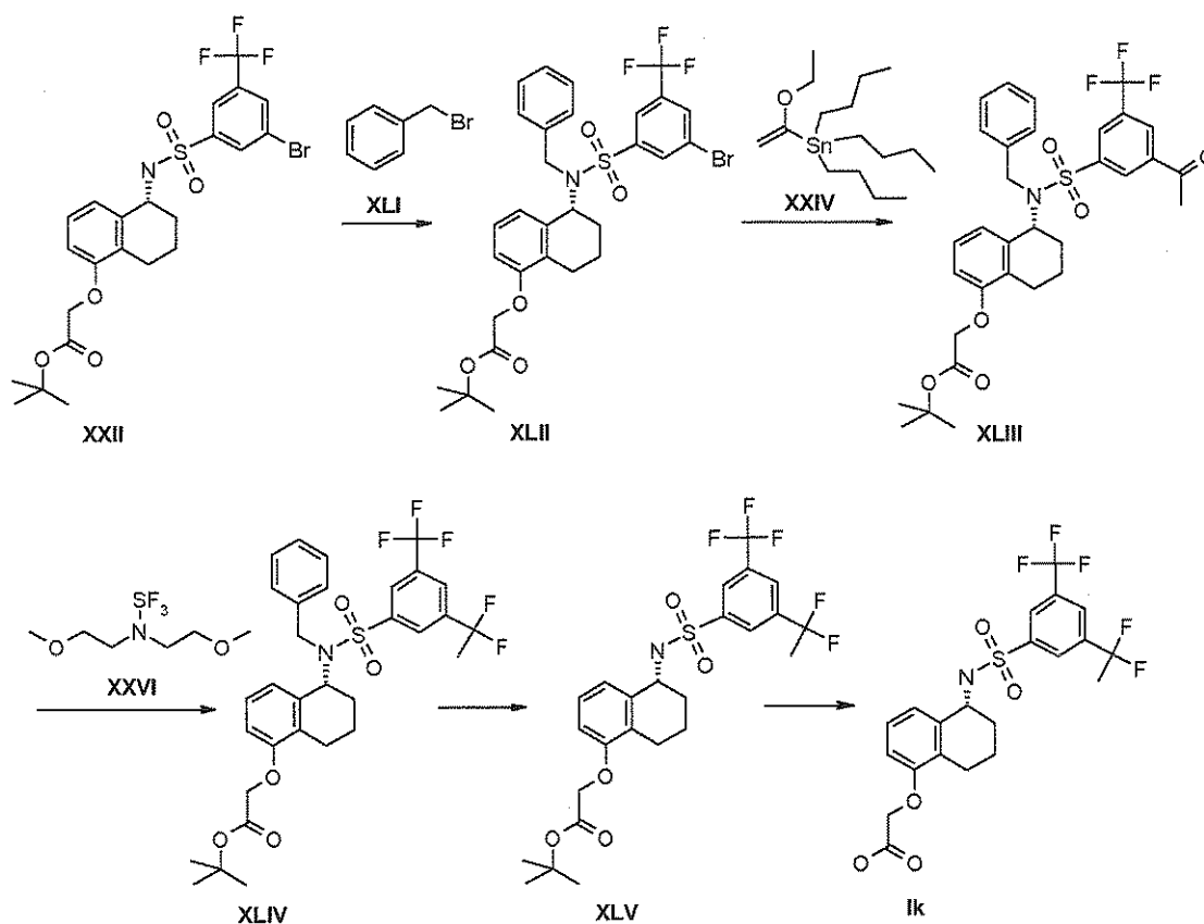
Scheme 10
