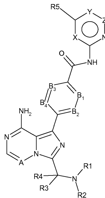
Formula I
