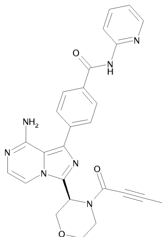
(R)-4-(8-Amino-3-(4-but-2-ynoylmorpholin-3-yl)imidazo[1,5-a]pyrazin-1-yl)-N-(pyridin-2-yl)benzamide
