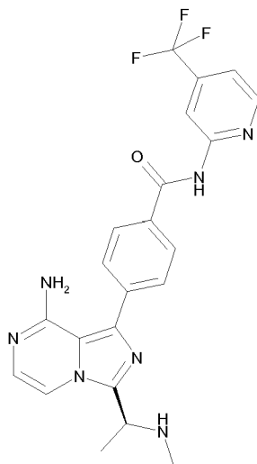
(S)-4-(8-Amino-3-(1-(methylamino)ethyl)imidazo[1,5-a]pyrazin-1-yl)-N-(4-(trifluoromethyl)pyridin-2-yl)benzamide
