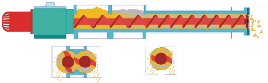
Drawing 2: single or twin screws
