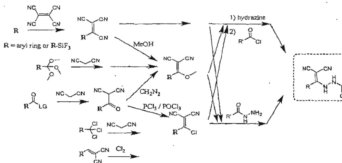
Scheme V:
