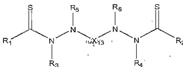
(XIII)
