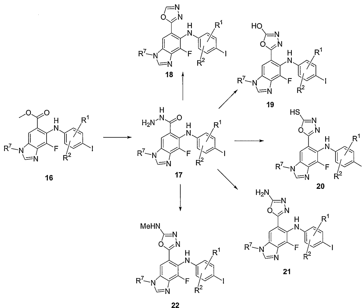
Scheme 3 – heterocyclic – oxadiazole example
