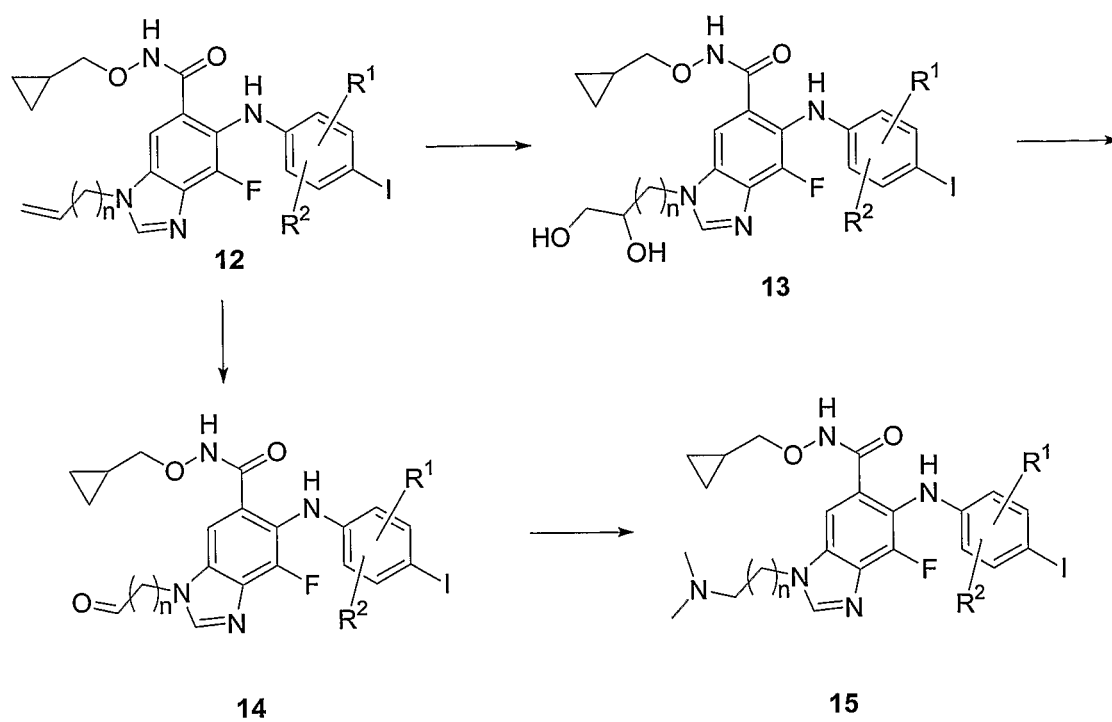
Scheme 2 – N amino alkyl iodo
