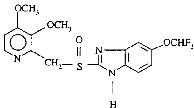
Pantoprazole
