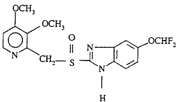
Pantoprazole
