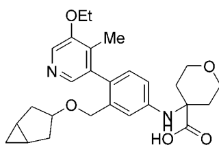
Compound 416
