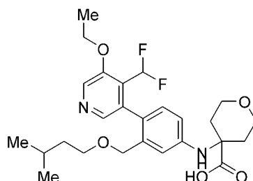
Synthesis of Compound 413: Step A: 2,6-dichloro-4-nitrobenzonitrile ( 2-1 ) reacts with EtOH, NaH in DMF at 0 °C - r.t. for 16 h to form ethyl 2-chloro-4-nitrobenzoate ( 2-2 ). Step B: 2-2 reacts with DIBAL-H in THF at -78 °C for 2 h to form ethyl 2-chloro-4-nitrobenzoate ( 2-3 ). Step C: 2-3 reacts with DAST in CH 2 Cl 2 at 0 °C - rt for 16 h to form ethyl 2-(difluoromethyl)-4-nitrobenzoate ( 2-4 ). Step D: 2-4 reacts with 1-bromo-3-iodobenzene ( 1-5 ) and 3-methylpentan-3-ol in t-BuOK, THF at 50 °C for 16 h to form ethyl 2-(difluoromethyl)-4-(3-methoxypropyl)benzoate ( 2-5 ). Step E: 2-5 reacts with 4-bromophenylhydrazide and CuI, DBU, DMA at 90 °C for 16 h to form ethyl 2-(difluoromethyl)-4-(3-methoxypropyl)benzoate ( 2-6 ). Step F: 2-6 reacts with MeI, K 2 CO 3 , DMF at 25 °C for 16 h to form ethyl 2-(difluoromethyl)-4-(3-methoxypropyl)benzoate ( 2-7 ). Step G: 2-7 reacts with Pd(dppf)Cl 2 , KOAc in dioxane at 100 °C for 16 h to form ethyl 2-(difluoromethyl)-4-(3-methoxypropyl)benzoate ( 2-8 ). Step H: 2-8 reacts with Catamount A-Pd-G 2 , K 2 CO 3 , THF, H 2 O at 100 °C for 16 h to form ethyl 2-(difluoromethyl)-4-(3-methoxypropyl)benzoate ( 2-9 ). Step I: 2-9 reacts with LiOH, MeOH, THF, H 2 O at 25 °C for 3 h to form ethyl 2-(difluoromethyl)-4-(3-methoxypropyl)benzoate ( Compound 413 ).
