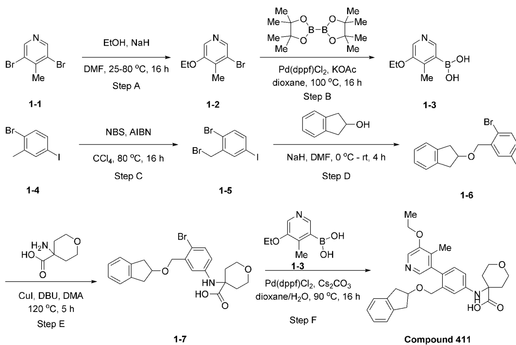
Compound 411
