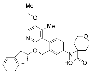
Compound 411
