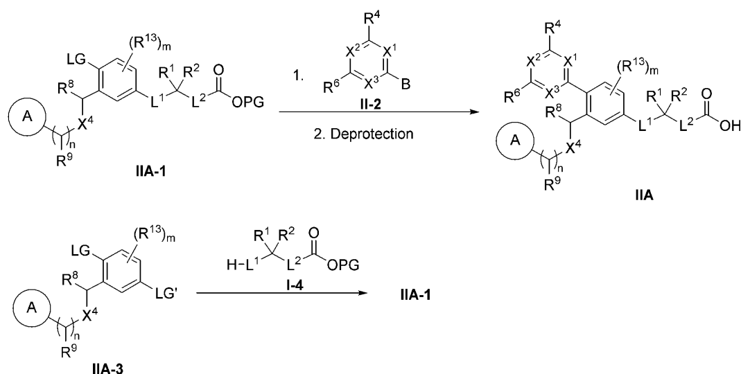
Scheme III
