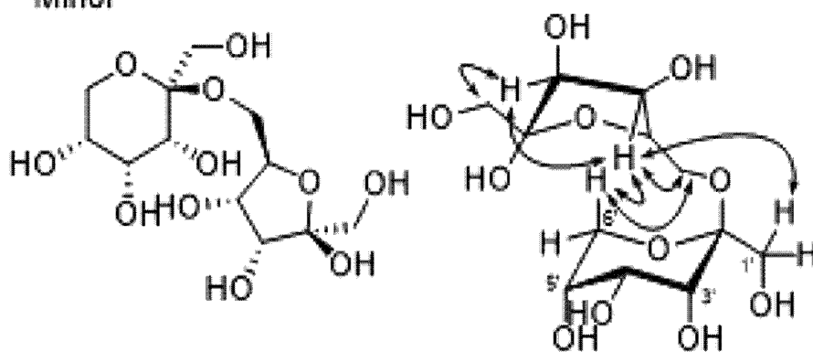
6-O-β-D-Psicopyranosyl-β-D-psicofuranose
