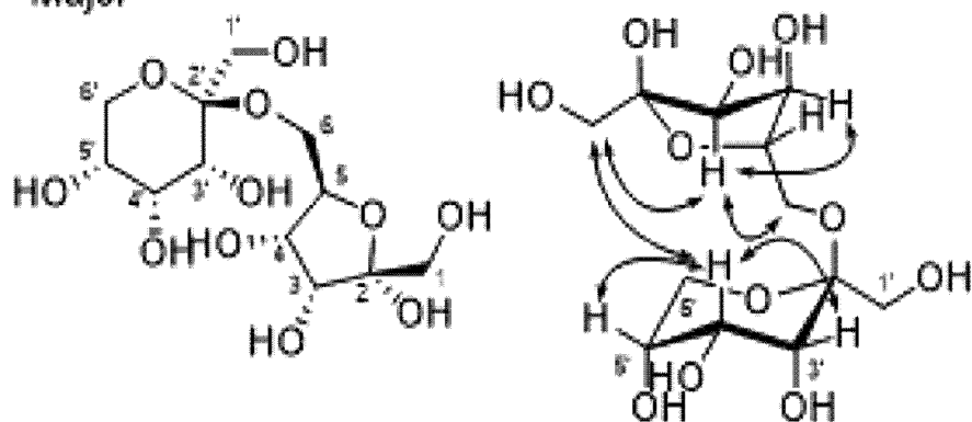
6-O-β-D-Psicopyranosyl-α-D-psicofuranose
