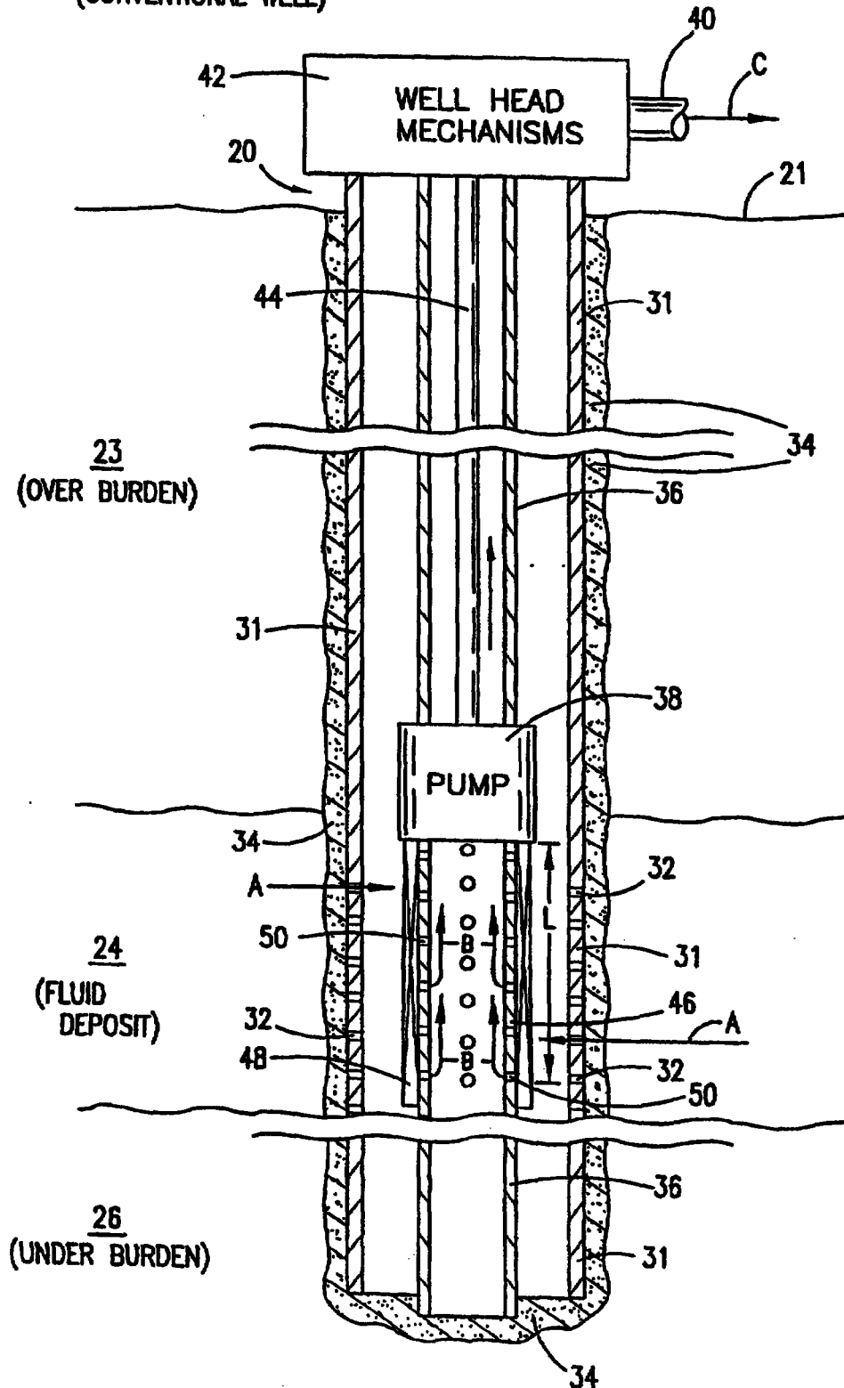
FIG. 1 (CONVENTIONAL WELL)
