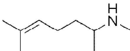
(6-methylamino-2-methylheptene)
