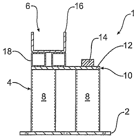
Figure 1 Section A-A
