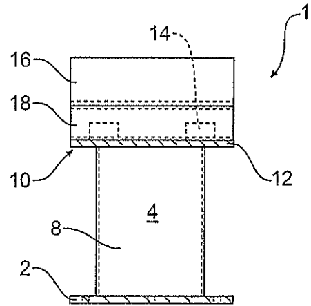
Figure 2 Section B-B
