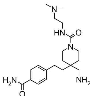
5 A.56 (Starting material: B.52)
