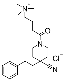
B.46 (Starting material: 3-Carboxy-propyl-trimethyl-ammonium chloride)
