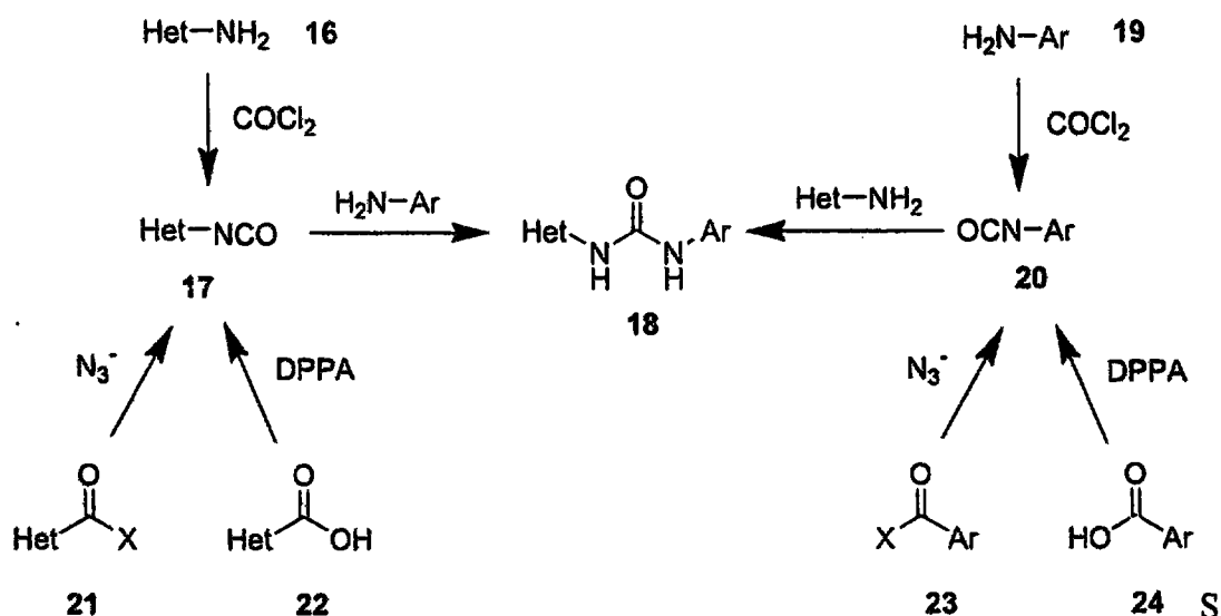
Scheme IV Selected Methods of Urea Formation (Het = heterocycle)
