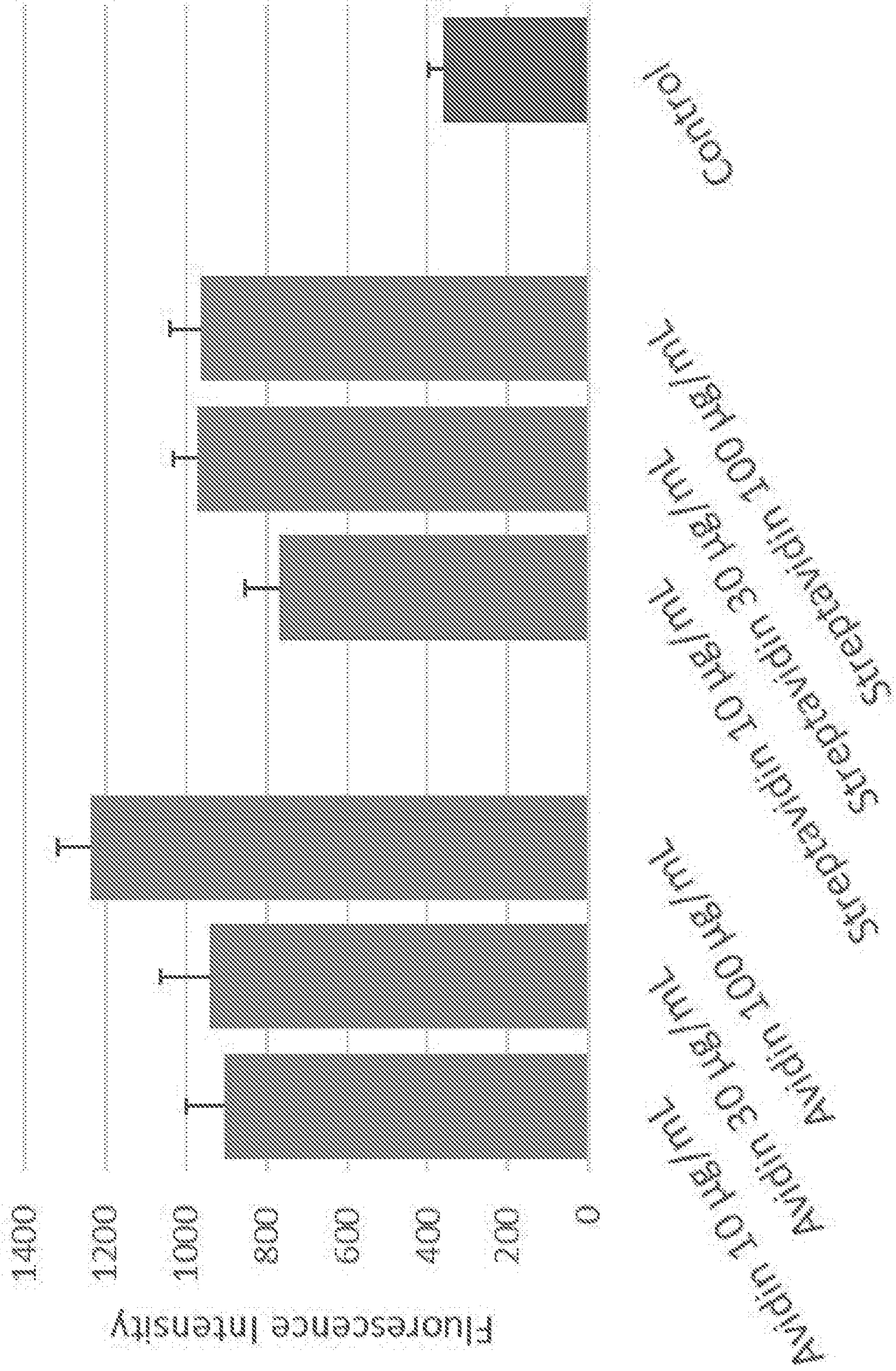
Comparison of Avidin and Streptavidin Coating
