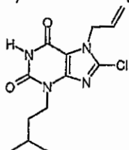
a) 8-chloro-3-(3-methylbutyl)-7-(2-propen-1-yl)-3,7-dihydro-1H-purine-2,6-dione
