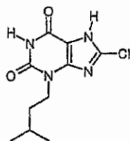
a) 8-chloro-3-(3-methylbutyl)-7-(2-propen-1-yl)-3,7-dihydro-1H-purine-2,6-dione
