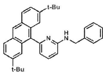
Ligand 1
