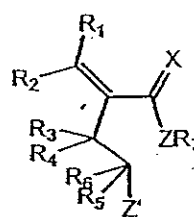
Formula Ib
