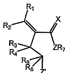
Formula Ib
