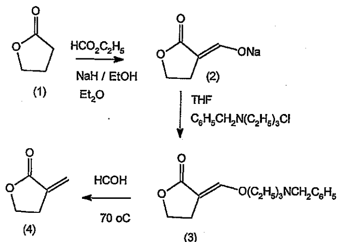
Scheme 4
