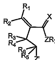
Formula Ib
