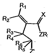
Formula Ib
