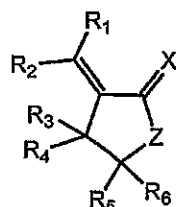
Formula Ia
