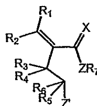
Formula Ib
