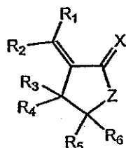
Formula Ia
