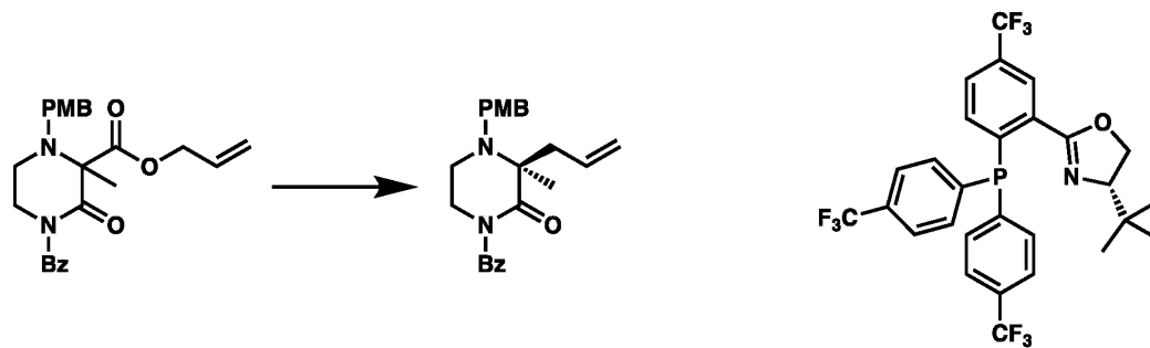
(S)-(p-CF 3 ) 3 -t-BuPHOX
