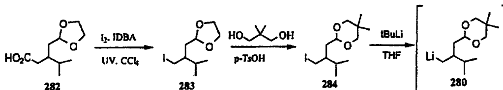
Scheme 72
