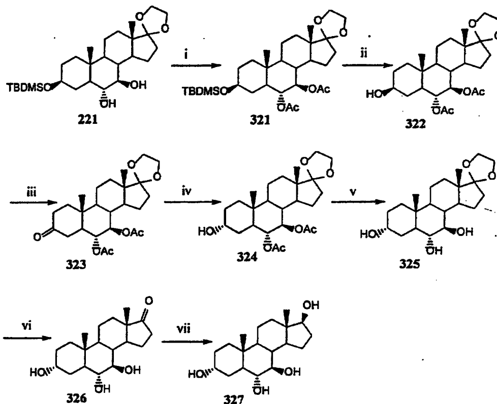
Scheme 76
