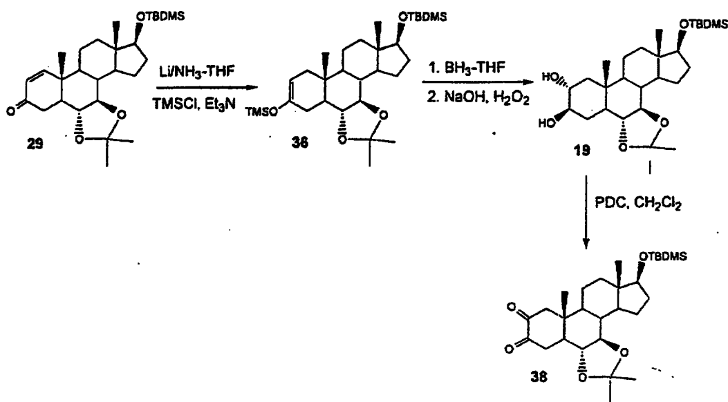
Scheme 9
