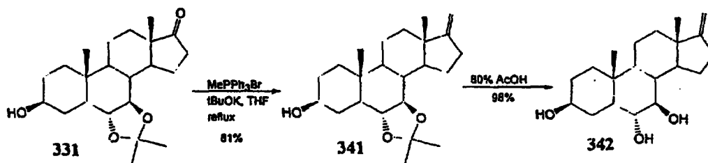
Scheme 87
