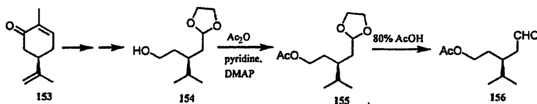
Scheme 45
