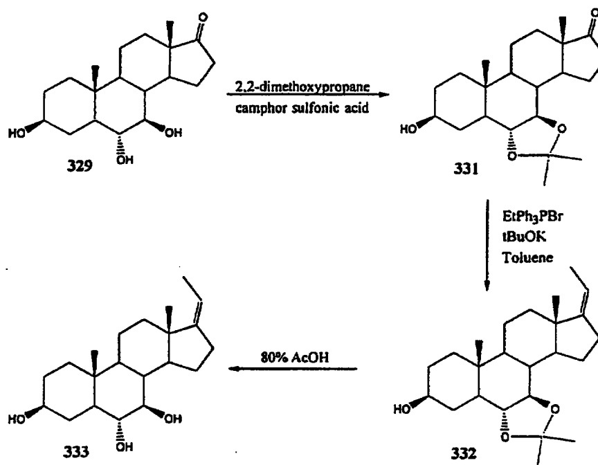
Scheme 80
