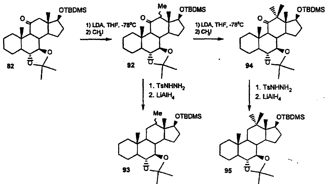
Scheme 27
