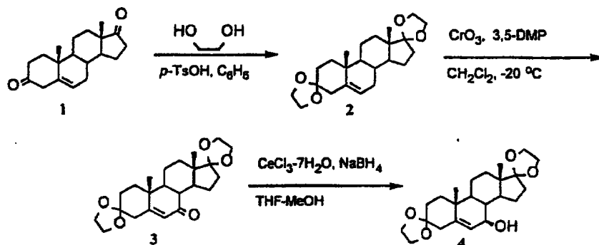
Scheme 56
