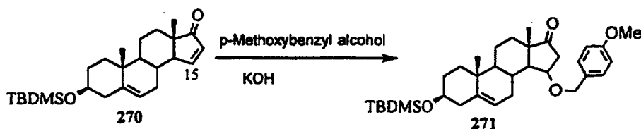
Scheme 67
