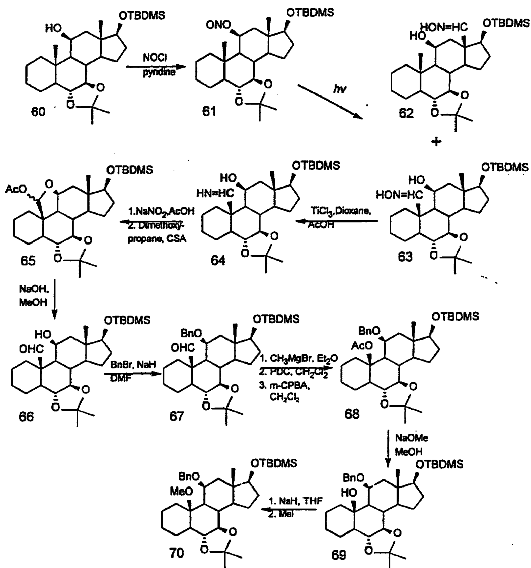
Scheme 20
