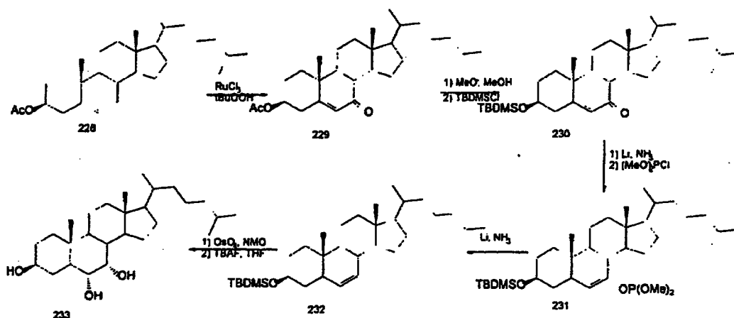
Scheme 54
