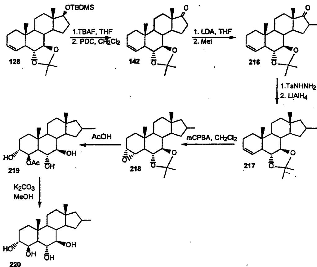
Scheme 52
