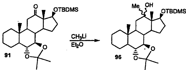
Scheme 28
