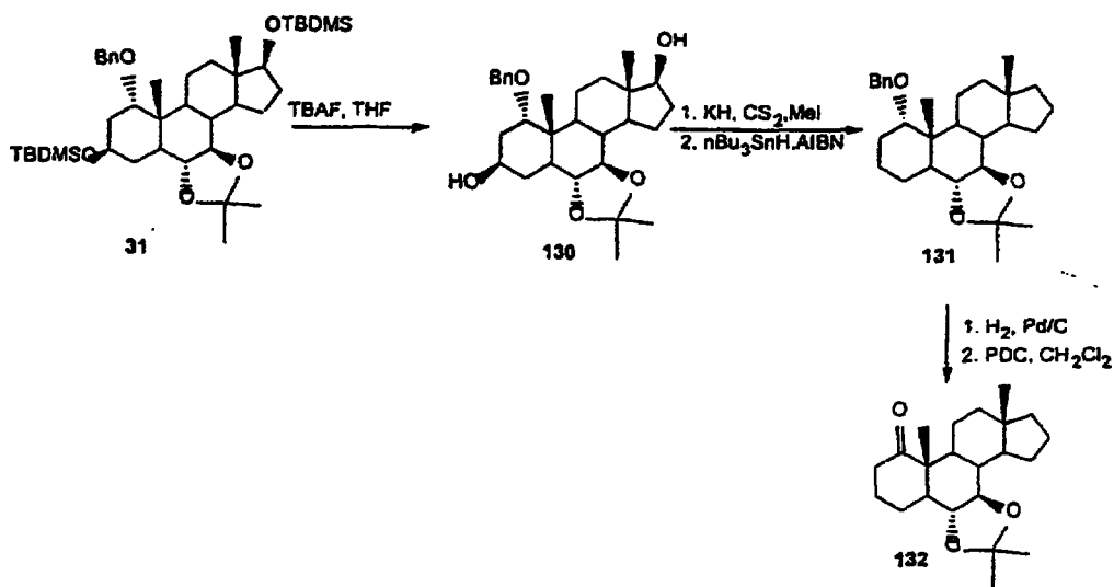
Scheme 41
