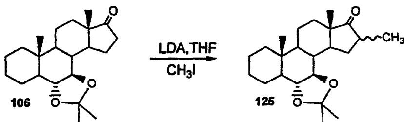
Scheme 37
