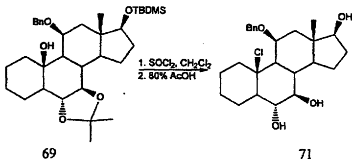
Scheme 21
