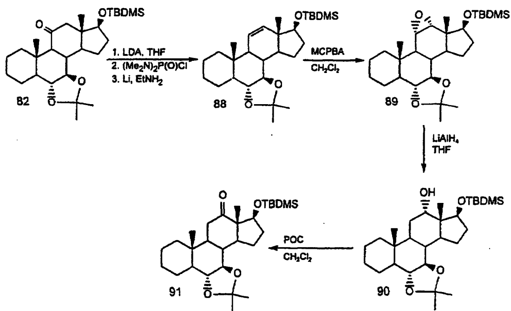
Scheme 26
