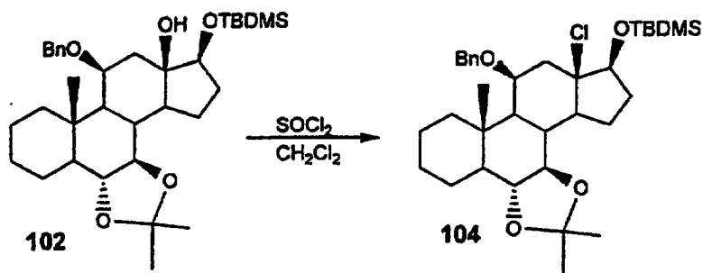
Scheme 30
