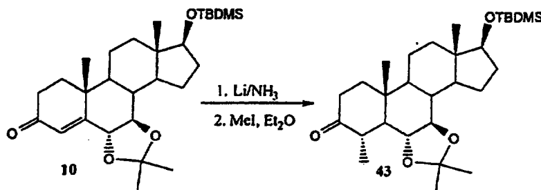
Scheme 12
