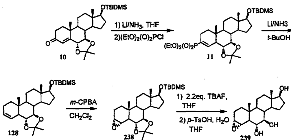
Scheme 60
