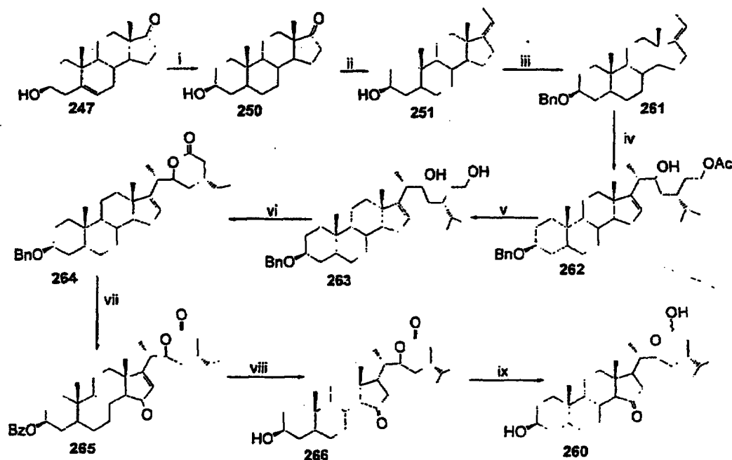
Scheme 65
