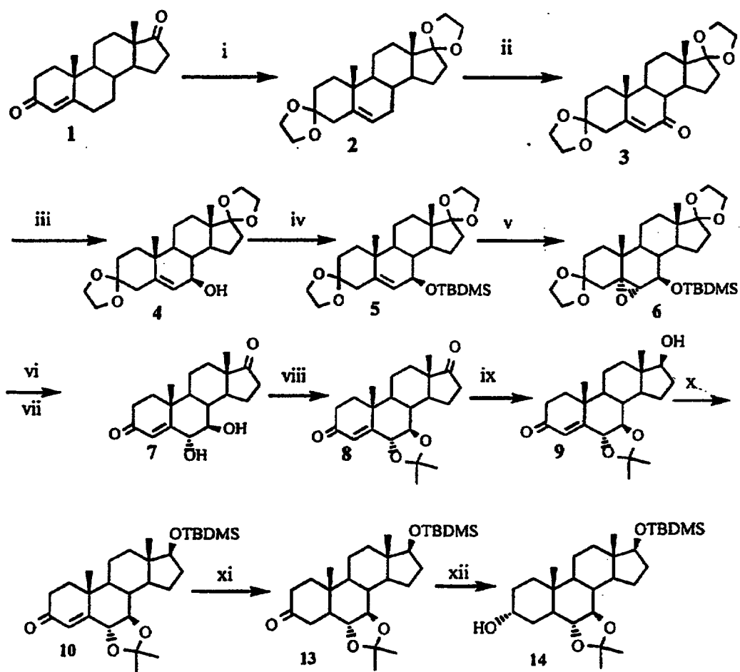
Scheme 79
