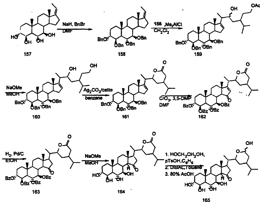
Scheme 46
