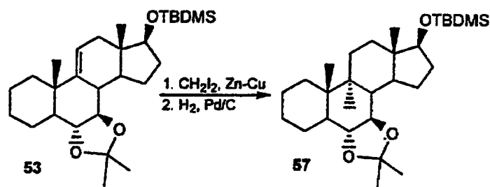
Scheme 18
