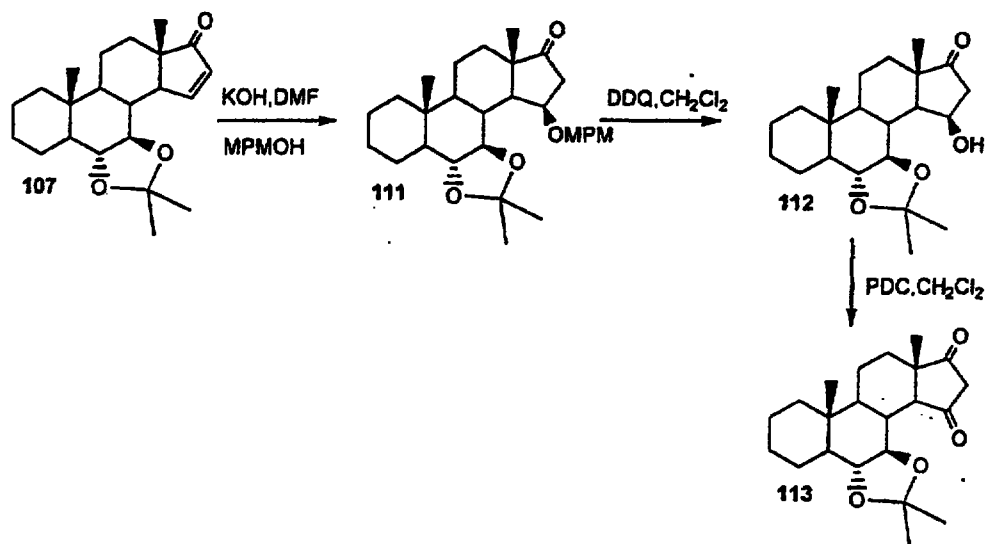
Scheme 32
