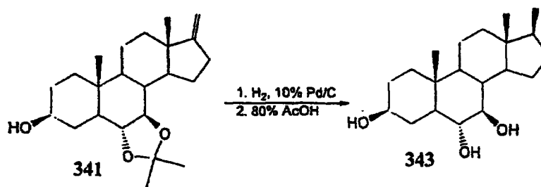
Scheme 87
