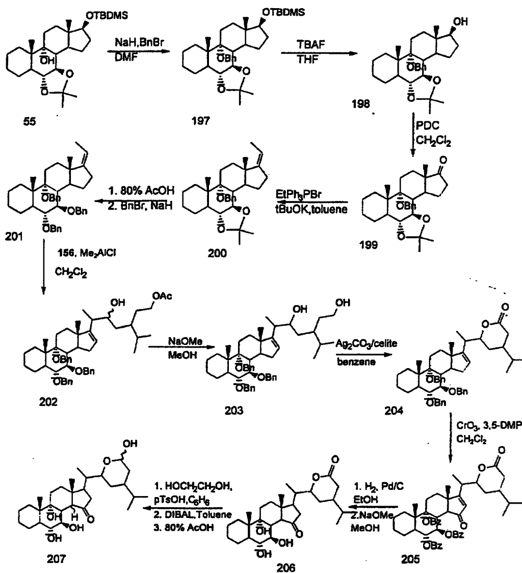
Scheme 50
