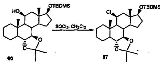
Scheme 25
