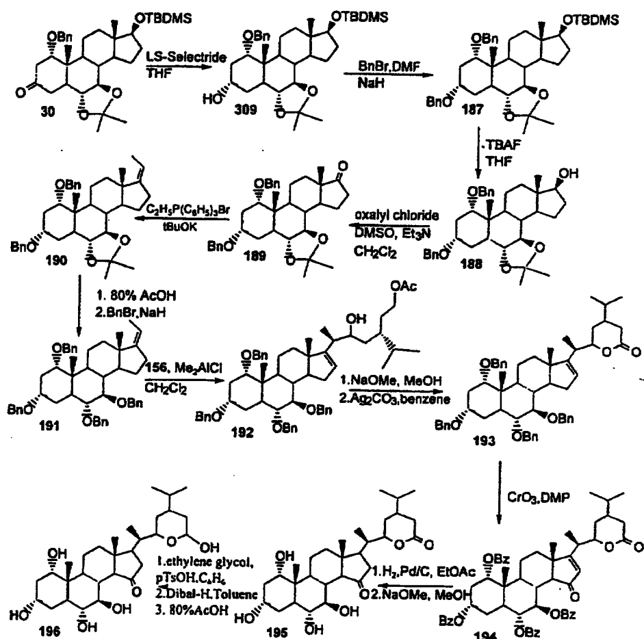
Scheme 49
