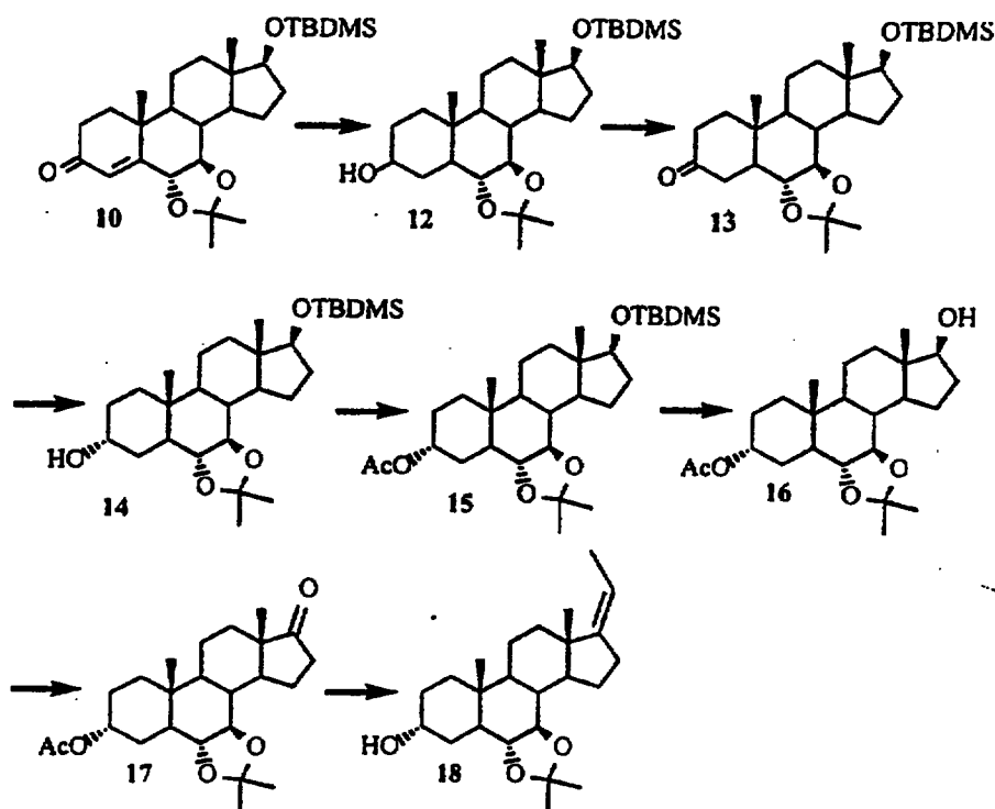
Scheme 3
