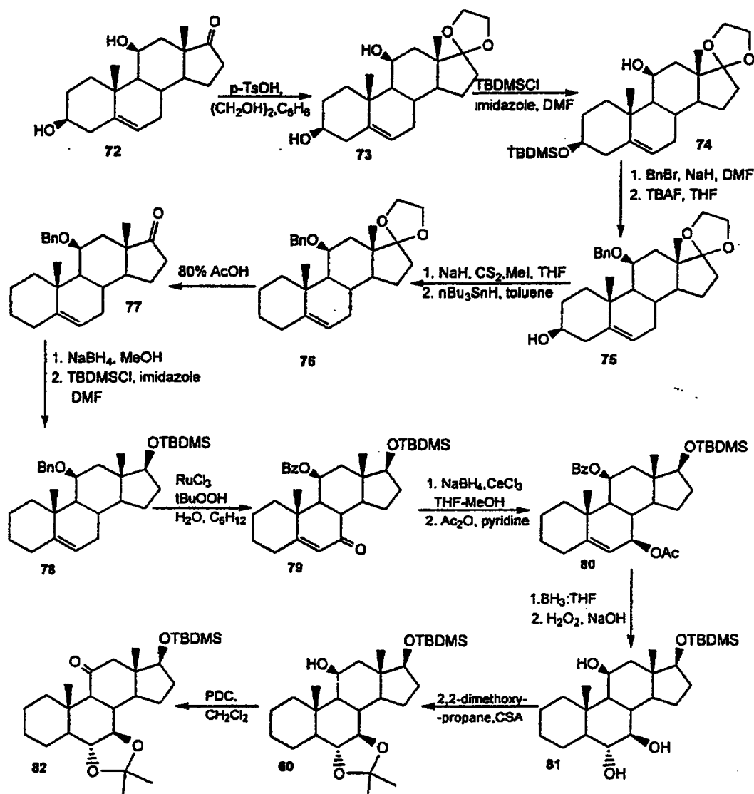
Scheme 22
