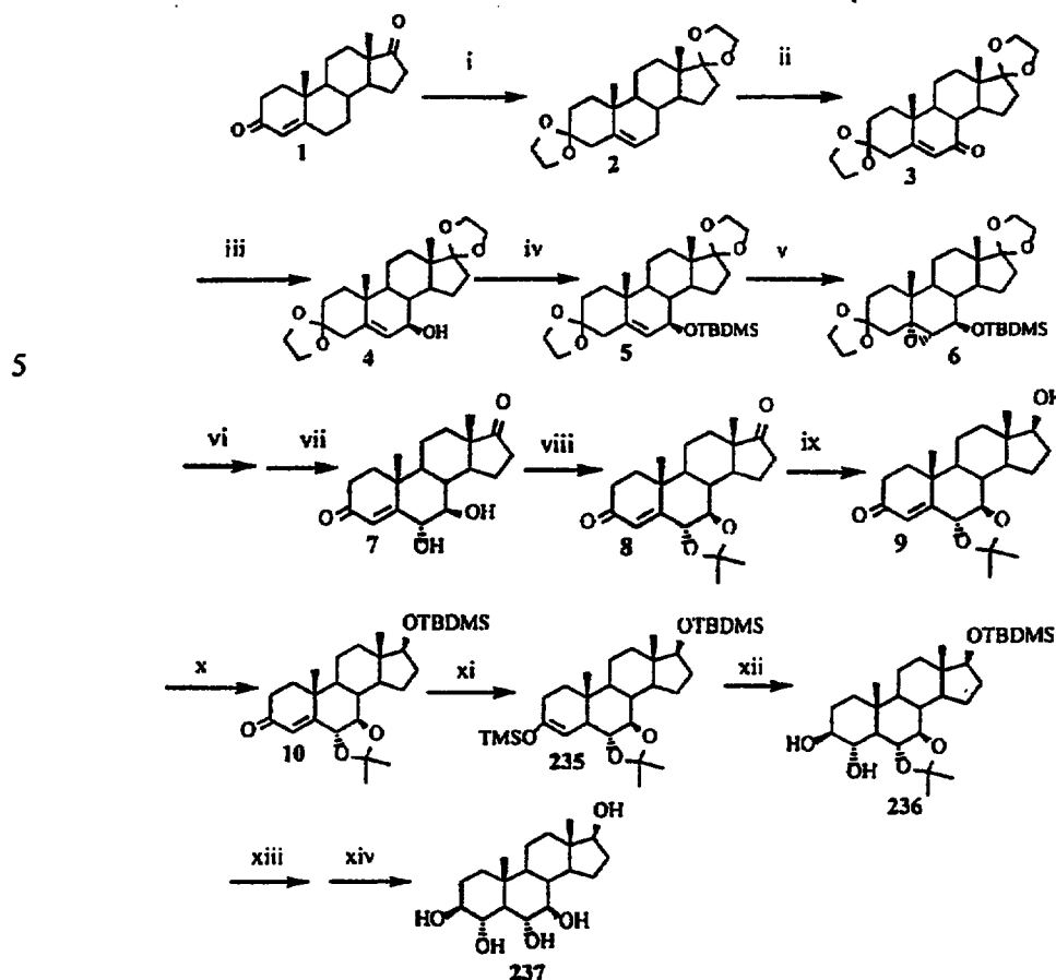
Scheme 55
