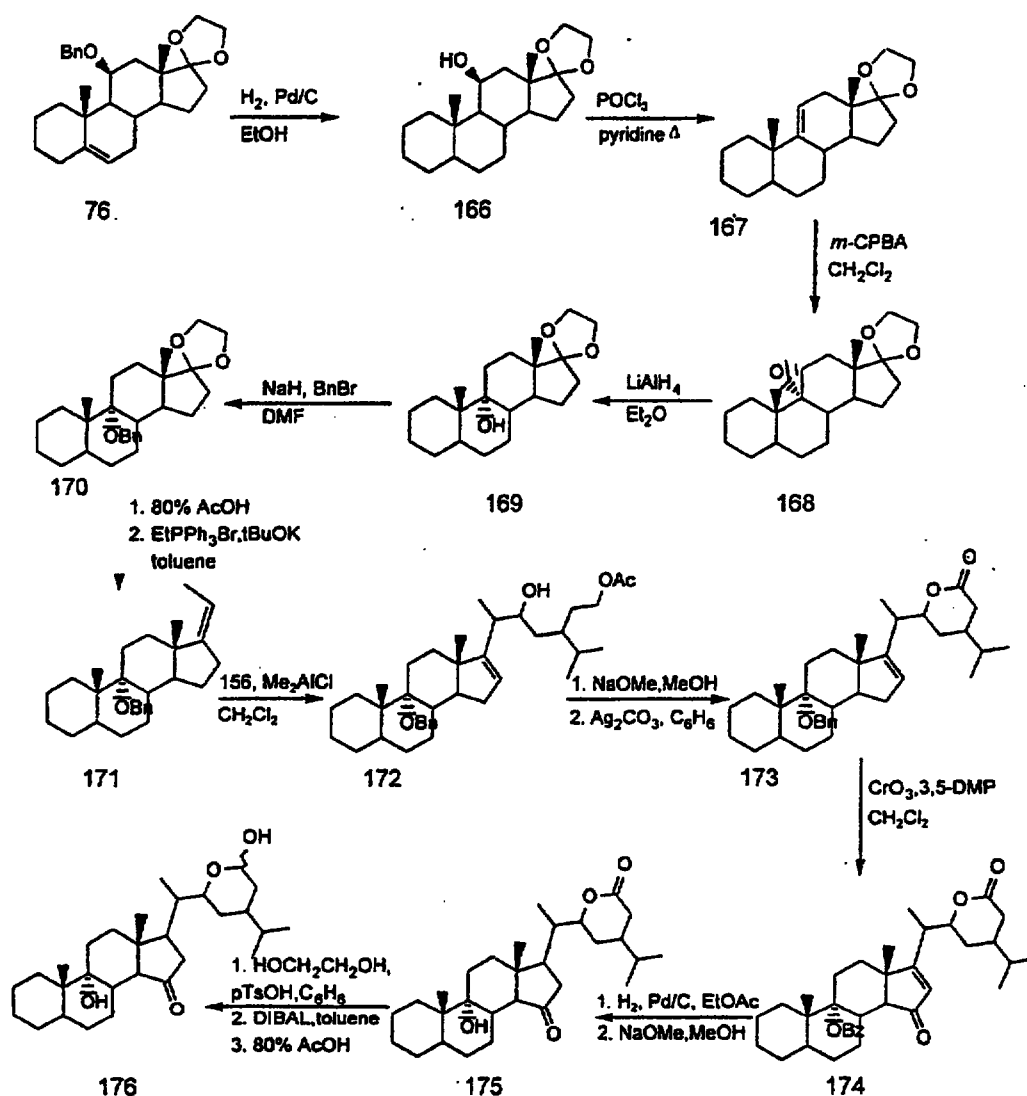
Scheme 47
