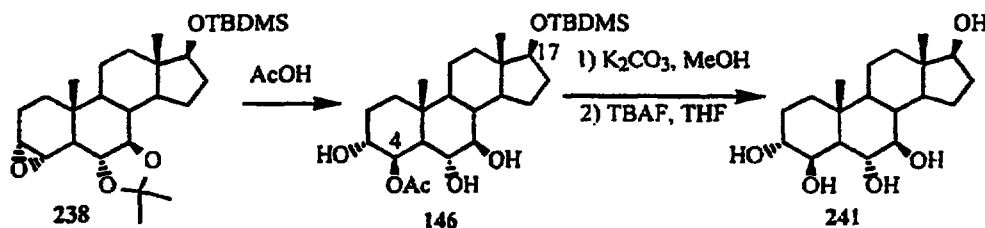
Scheme 62
