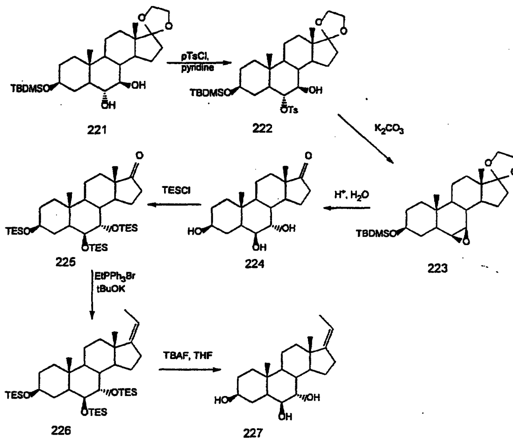
Scheme 53
