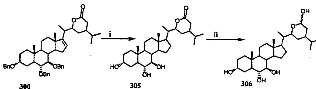
Scheme 74
