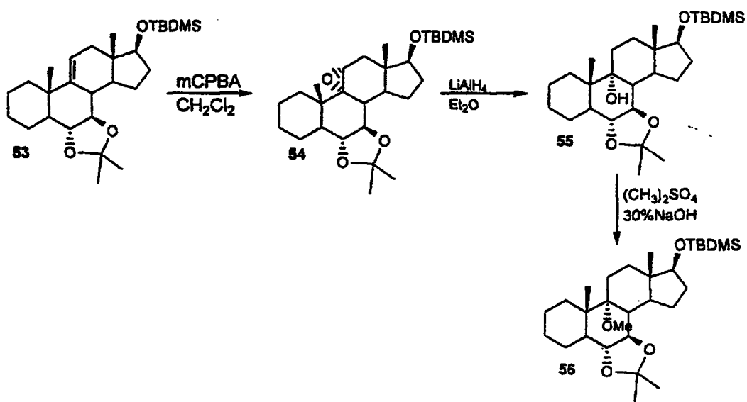
Scheme 17
