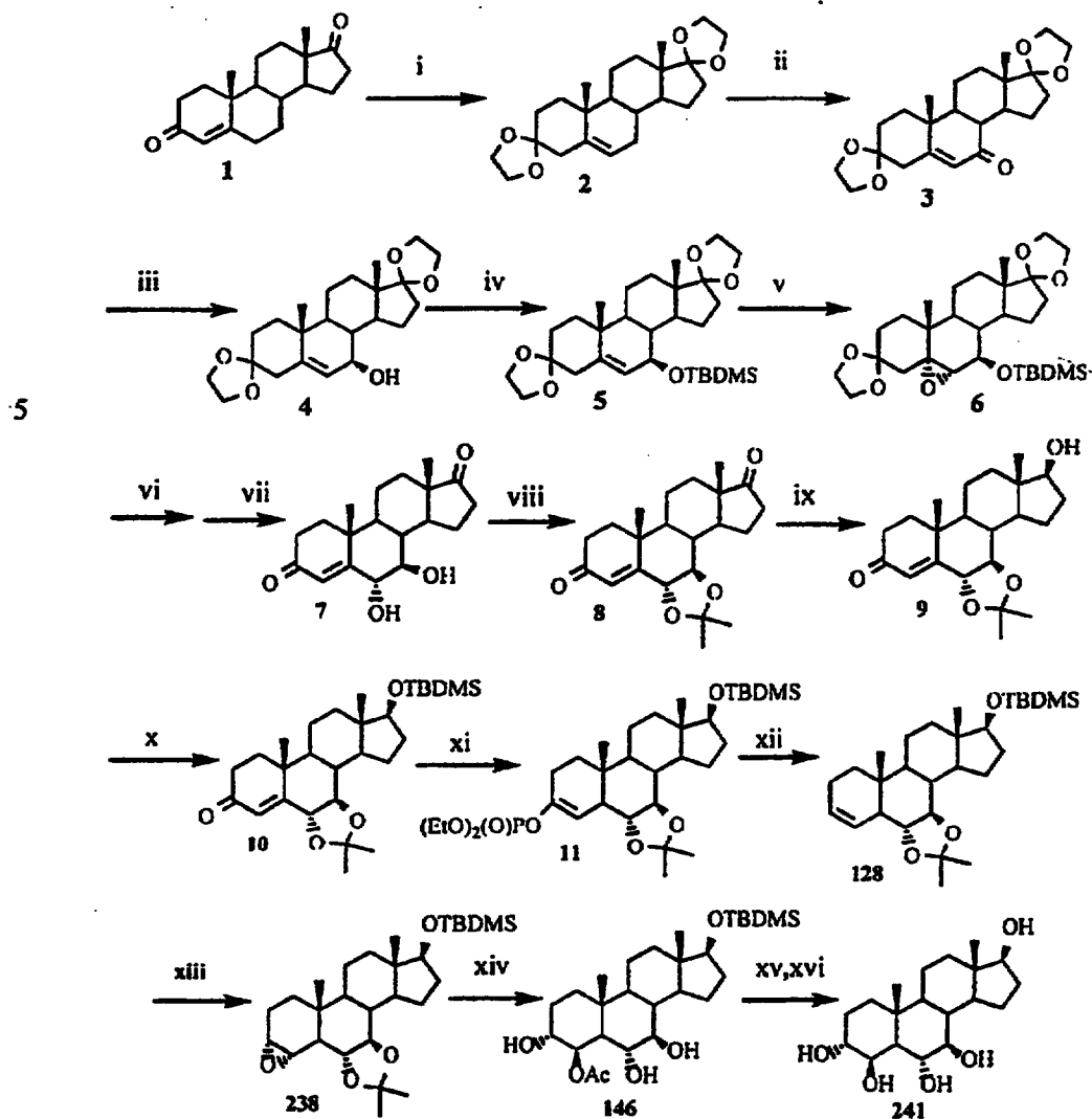
Scheme 61
