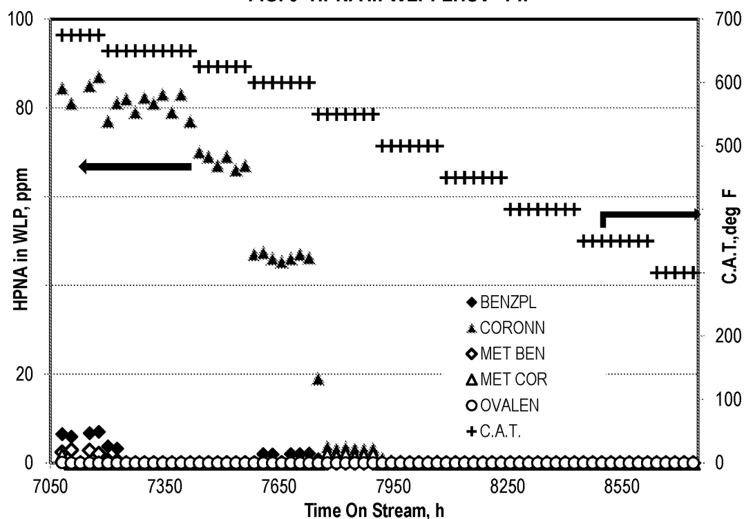
FIG. 9 HPNA in WLP: LHSV=1 h -1
