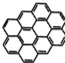
Ovalene
