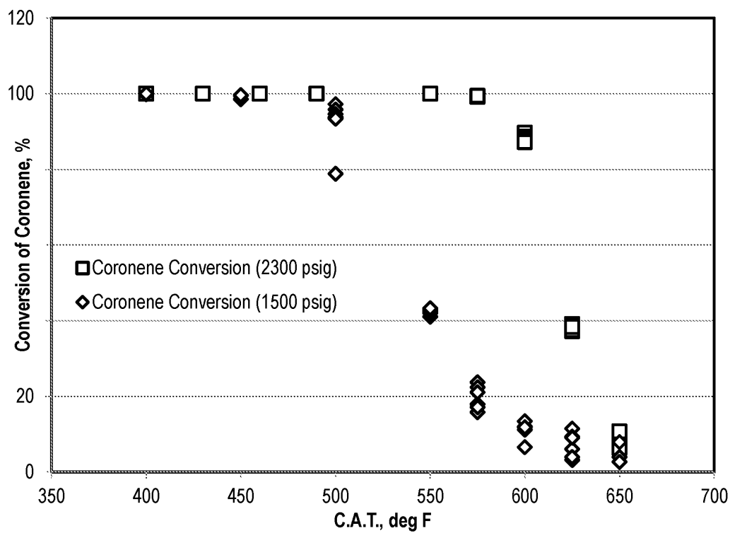
FIG. 11 Coronene Conversion (2300 &amp; 1500 psig)
