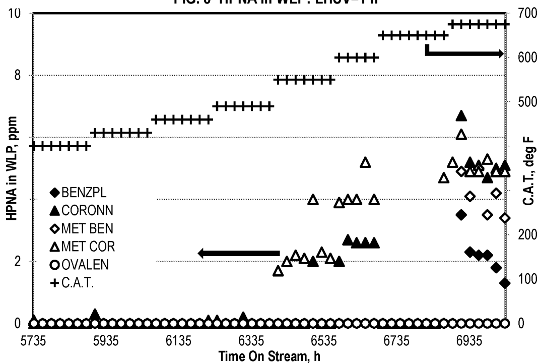
FIG. 9 HPNA in WLP: LHSV=1 h -1
