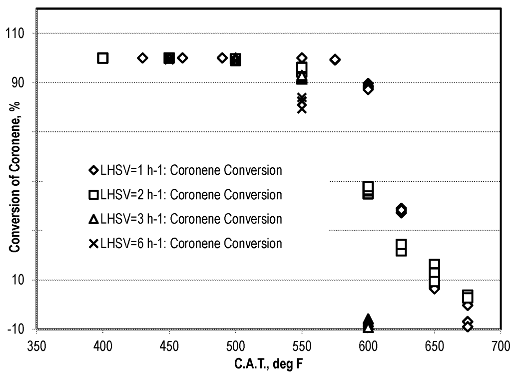
FIG. 10 Coronene Conversion vs LHSV
