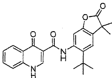
Compound 21
