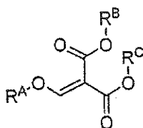
Formula 51
