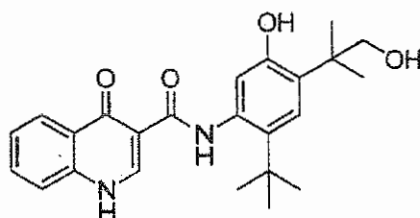
Compound 27
