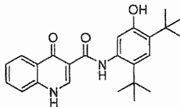
Compound 34
