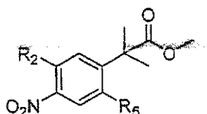
Formula 42 , wherein
