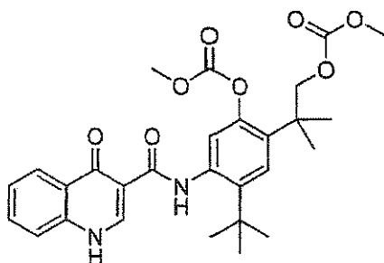
Compound 14
