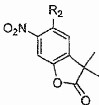
Formula 45 , wherein
