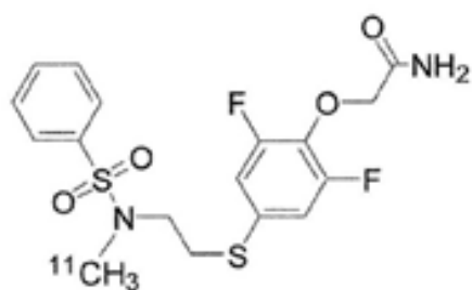
Radio-labeled K-2
