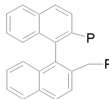
2, 2' Binaphthyl
