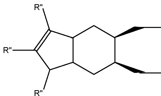
substituted 3a,
