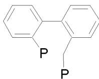
2, 2', Biphenyl
