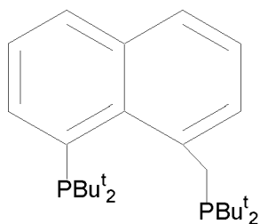
1-(di-tert-butylphosphino)-8-(di-tertbutylphosphinomethyl)-naphthalene
