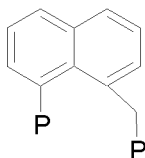
1, 8, Naphthyl
