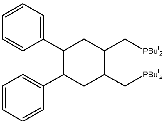
cis-1,2-bis(di-tert-butylphosphinomethyl)-4,5-diphenylcyclohexane
