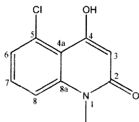
5-chloro-4-hydroxy-1-methylquinolin-2(1H)-one Chemical Formula: C 10 H 8 ClNO 2 Molecular Weight: 209.629
