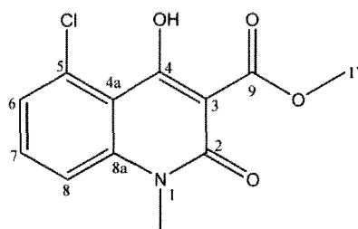
methyl 5-chloro-4-hydroxy-1-methyl-2-oxo-1,2-dihydroquinoline-3-carboxylate
