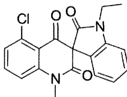
1H,3H-spiro[5-chloro-1-methylquinoline-2,4-dione-3,3'-[1]ethylindolin-[2]-one] Chemical Formula: C 19 H 13 ClN 2 O 3 Molecular Weight: 354.787
