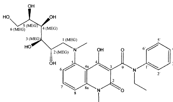
N -ethyl-4-hydroxy-1-methyl-5-(2,3,4,5,6-pentahydroxyhexylamino)-2-oxo- N -phenyl-1,2-dihydroquinoline-3-carboxamide Chemical Formula: C 26 H 33 N 3 O 8 Molecular Weight: 515.556
