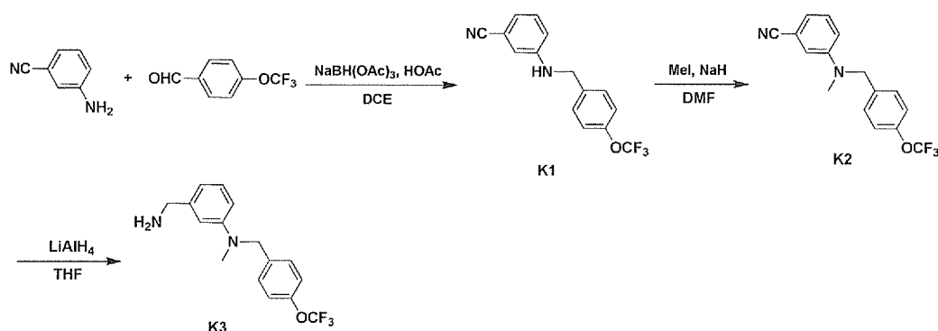
Scheme 11
