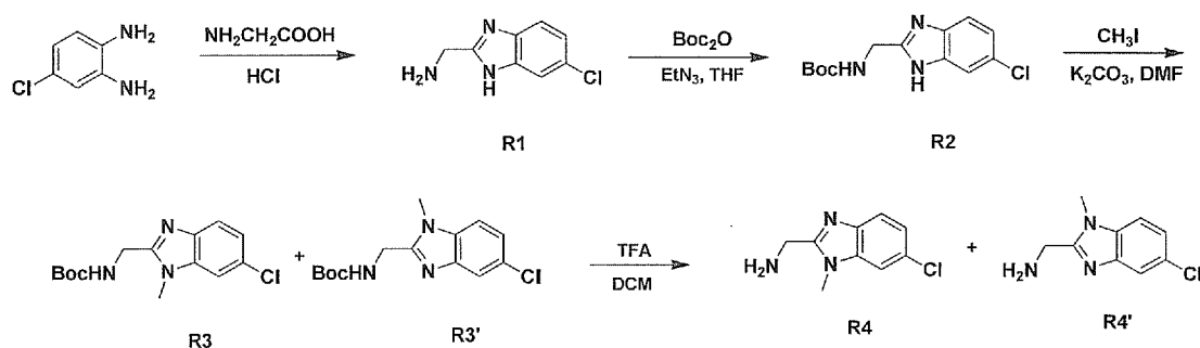
Scheme 18
