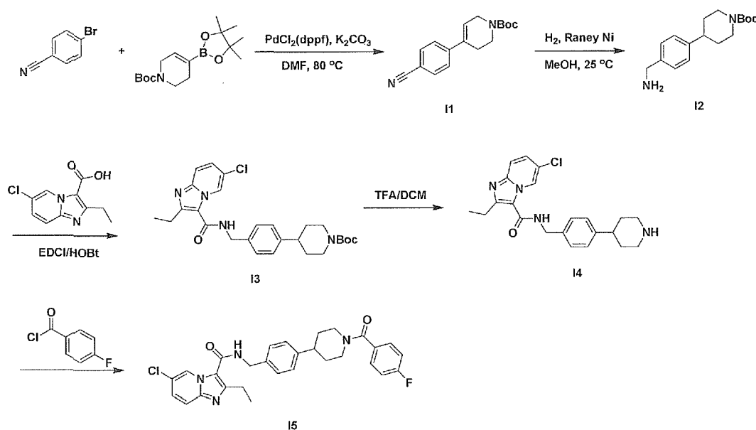
Scheme 9
