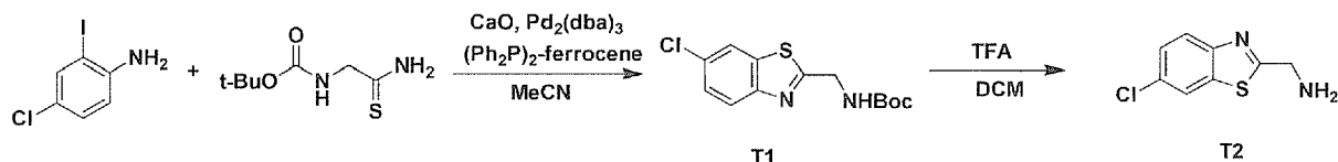
Scheme 20
