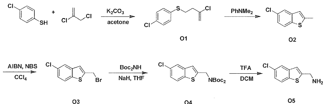
Scheme 15
