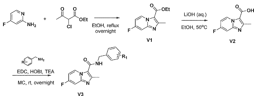
Scheme 22
