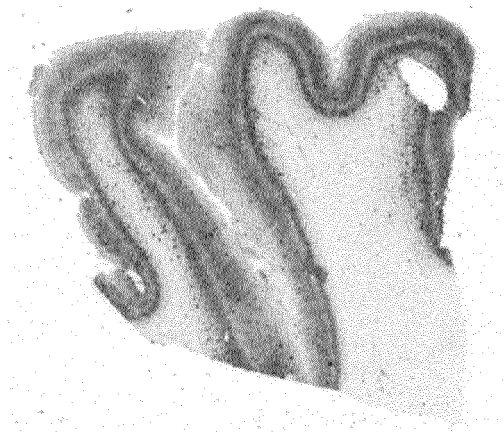
Autoradiogram of 3 H-2-(6-fluoro-pyridin-3-yl)-9H-dipyrido[2,3-b;3',4'-d]pyrrole
