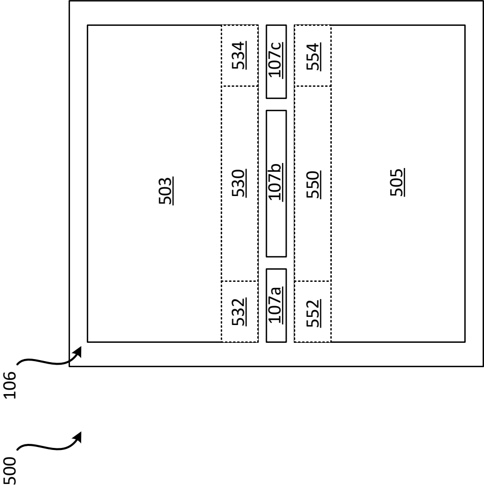
PLAN VIEW FIG. 5
