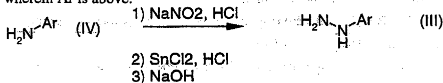
Scheme 2. The hydrazines
