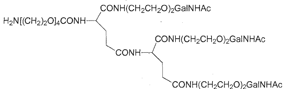
Compound VII
