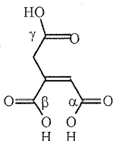
aconitic acid
