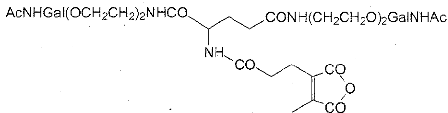
Compound VI
