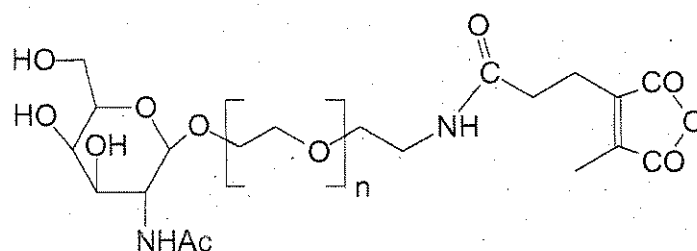
Compound II
