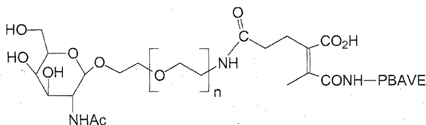
Compound III
