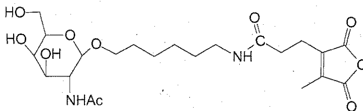
Compound V
