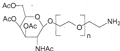
Compound I
