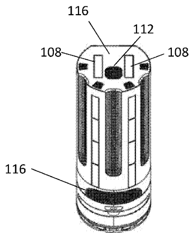
Figure 1e (perspective)
